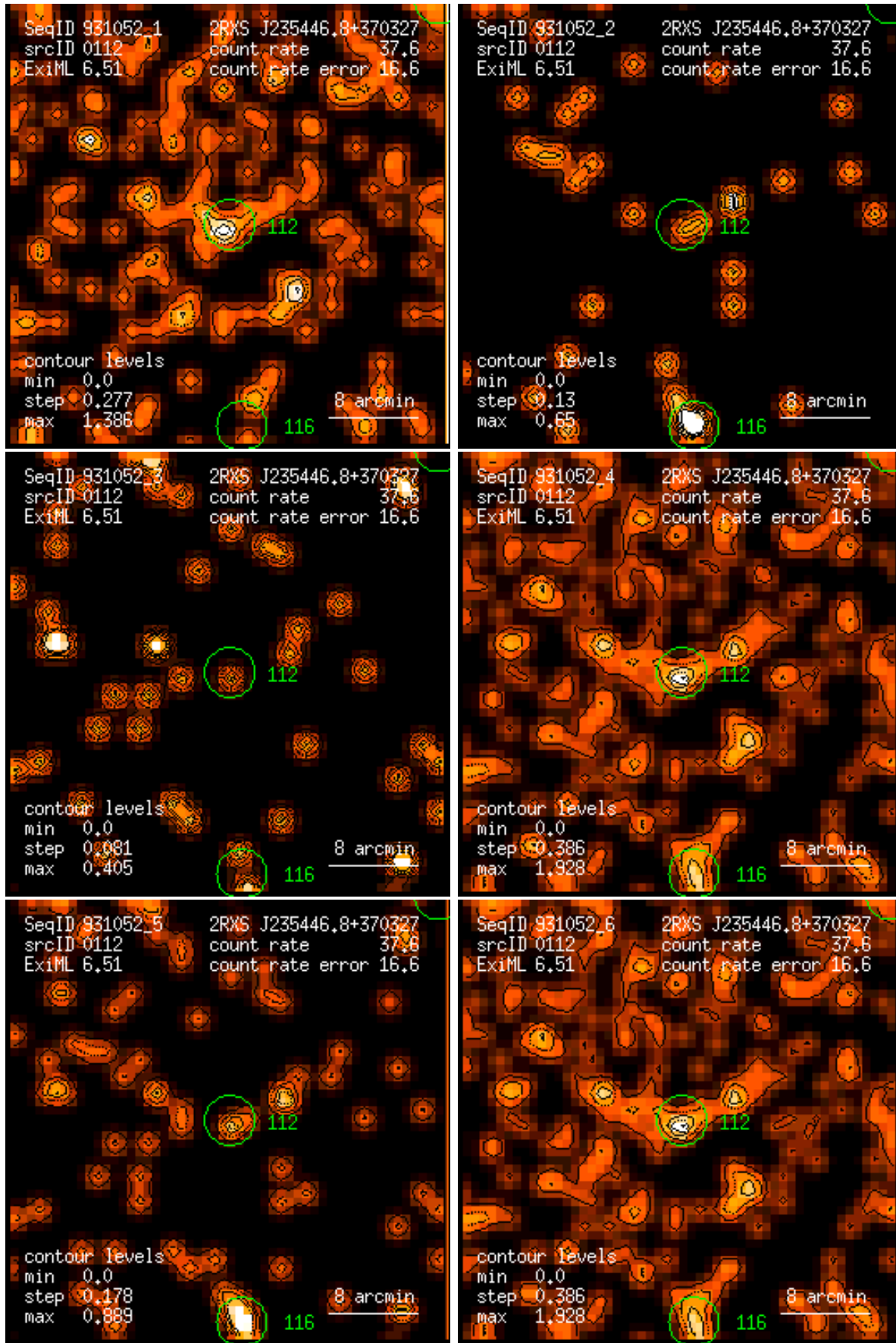
Figure 112: RASS 931052: detection 0112: band rate images, Gaussian filter: (1) PSPC channels 11 – 41, (2) 52 – 90, (3) 91 – 201, (4) 11 – 235, (5) 52 – 201, (6) 11 – 201. Broad band rates in counts/ks. Band rate contour levels in counts/ks/arcmin 2 .
