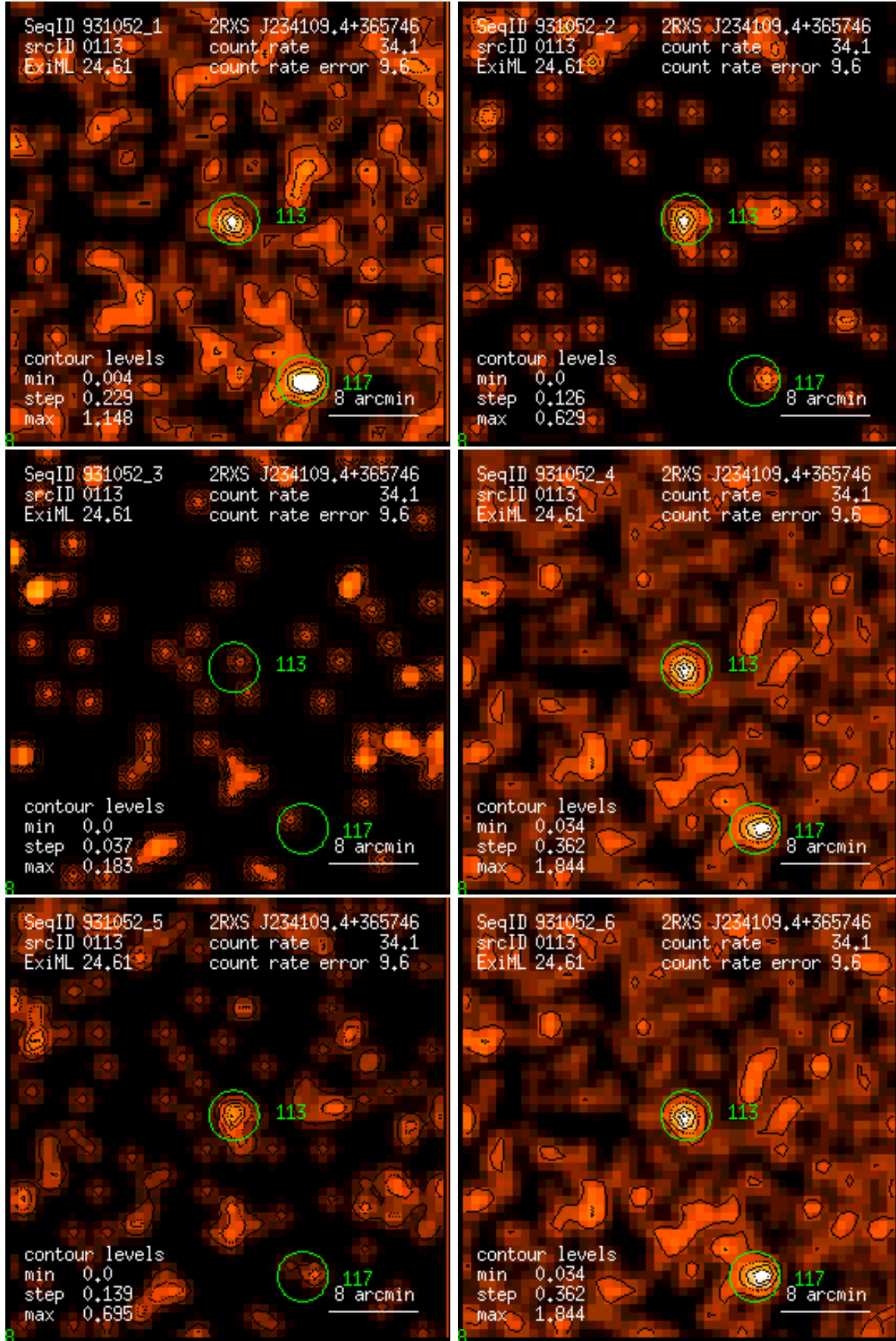
Figure 113: RASS 931052: detection 0113: band rate images, Gaussian filter: (1) PSPC channels 11 – 41, (2) 52 – 90, (3) 91 – 201, (4) 11 – 235, (5) 52 – 201, (6) 11 – 201. Broad band rates in counts/ks. Band rate contour levels in counts/ks/arcmin 2 .
