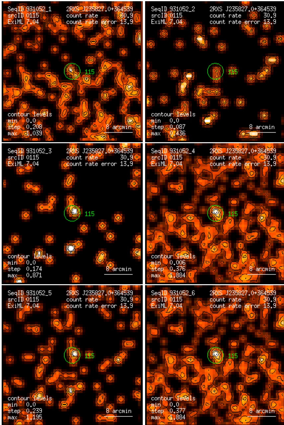
Figure 115: RASS 931052: detection 0115: band rate images, Gaussian filter: (1) PSPC channels 11 – 41, (2) 52 – 90, (3) 91 – 201, (4) 11 – 235, (5) 52 – 201, (6) 11 – 201. Broad band rates in counts/ks. Band rate contour levels in counts/ks/arcmin 2 .
