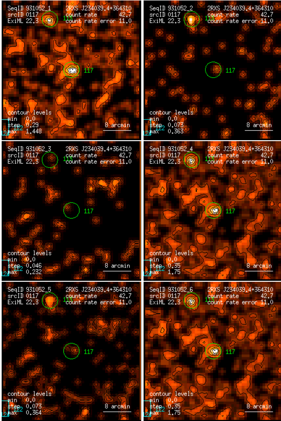
Figure 117: RASS 931052: detection 0117: band rate images, Gaussian filter: (1) PSPC channels 11 – 41, (2) 52 – 90, (3) 91 – 201, (4) 11 – 235, (5) 52 – 201, (6) 11 – 201. Broad band rates in counts/ks. Band rate contour levels in counts/ks/arcmin 2 .
