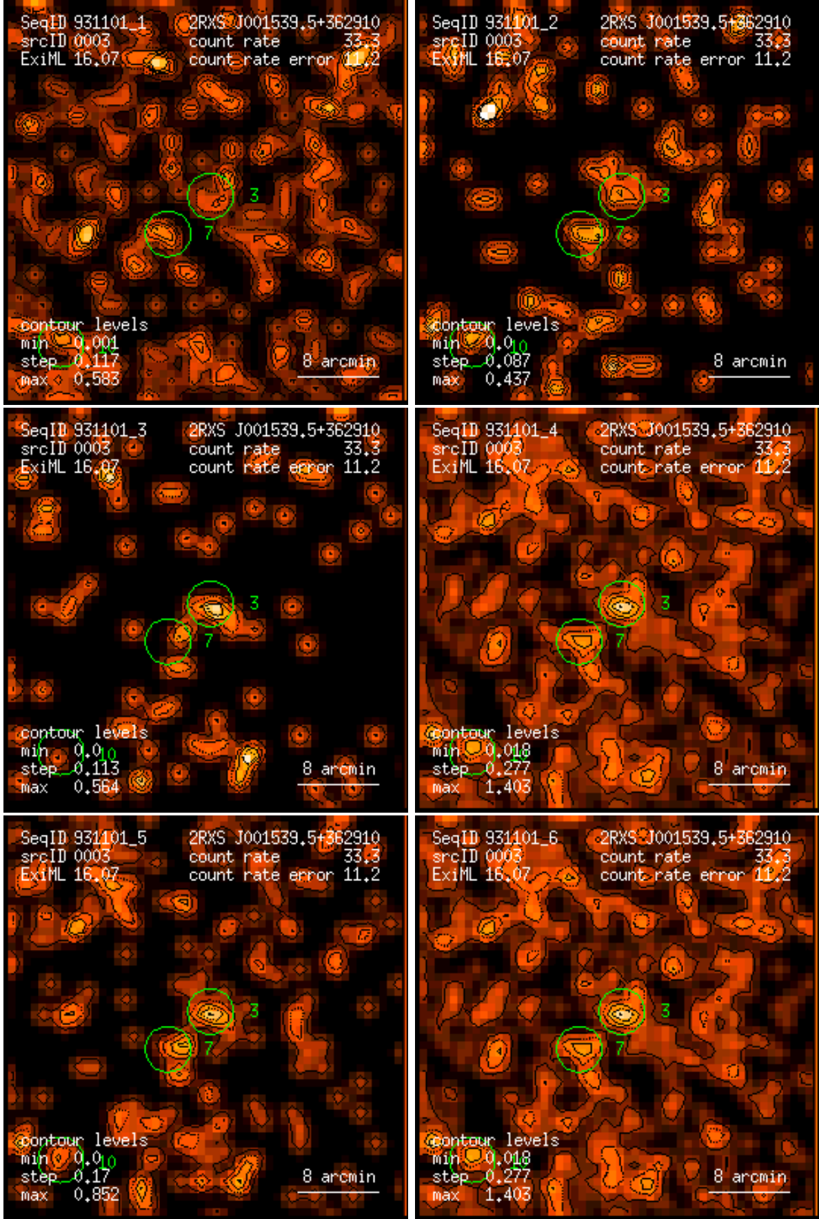
Figure 3: RASS 931101: detection 0003: band rate images, Gaussian filter: (1) PSPC channels 11 – 41, (2) 52 – 90, (3) 91 – 201, (4) 11 – 235, (5) 52 – 201, (6) 11 – 201. Broad band rates in counts/ks. Band rate contour levels in counts/ks/arcmin 2 .
