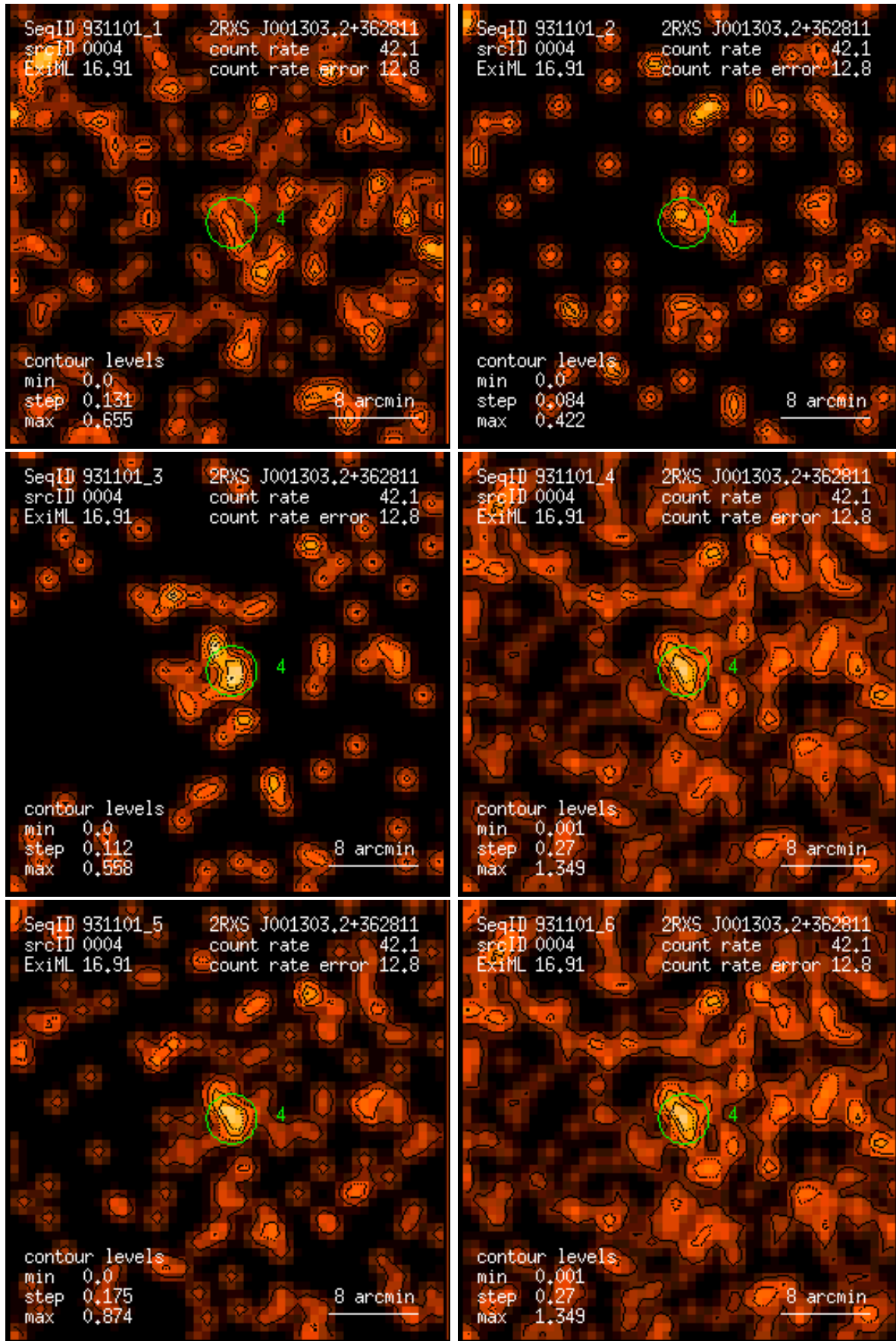
Figure 4: RASS 931101: detection 0004: band rate images, Gaussian filter: (1) PSPC channels 11 – 41, (2) 52 – 90, (3) 91 – 201, (4) 11 – 235, (5) 52 – 201, (6) 11 – 201. Broad band rates in counts/ks. Band rate contour levels in counts/ks/arcmin 2 .
