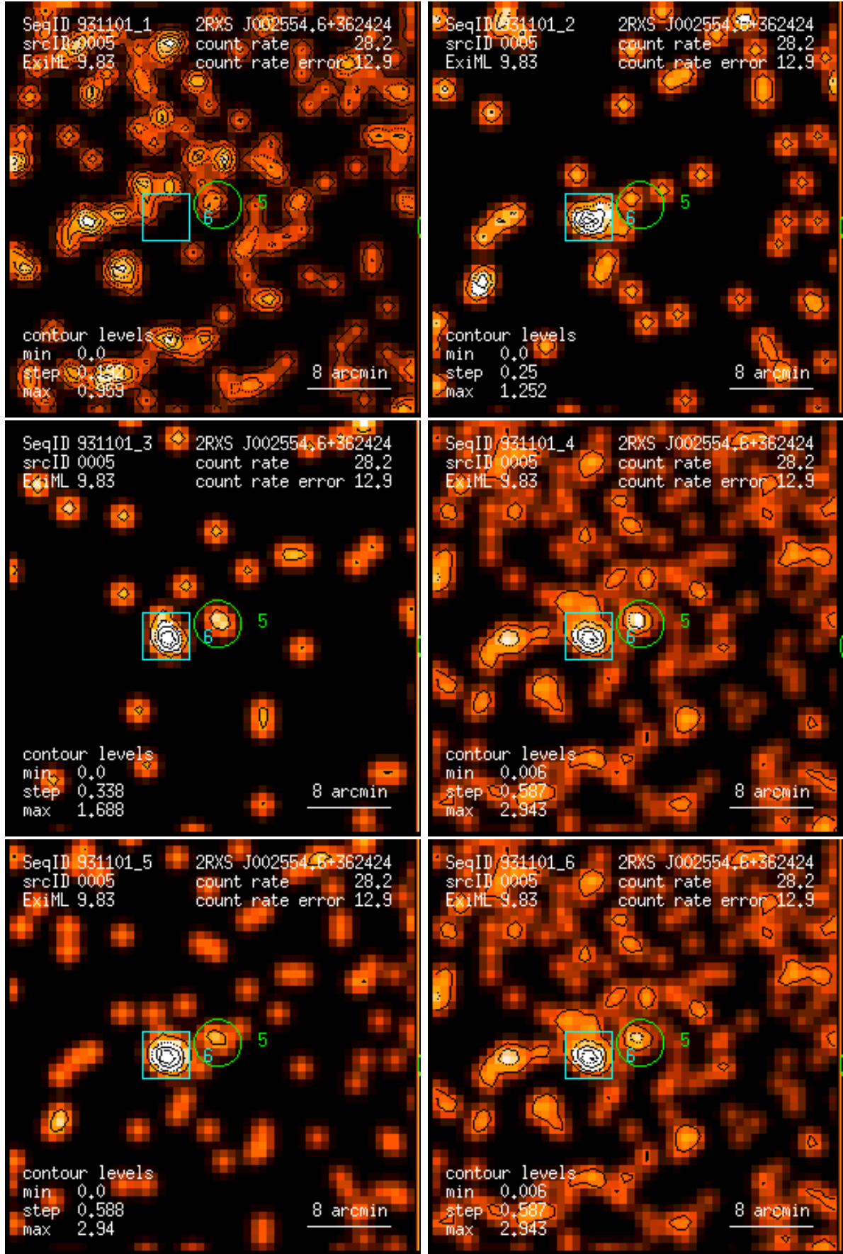
Figure 5: RASS 931101: detection 0005: band rate images, Gaussian filter: (1) PSPC channels 11 – 41, (2) 52 – 90, (3) 91 – 201, (4) 11 – 235, (5) 52 – 201, (6) 11 – 201. Broad band rates in counts/ks. Band rate contour levels in counts/ks/arcmin 2 .
