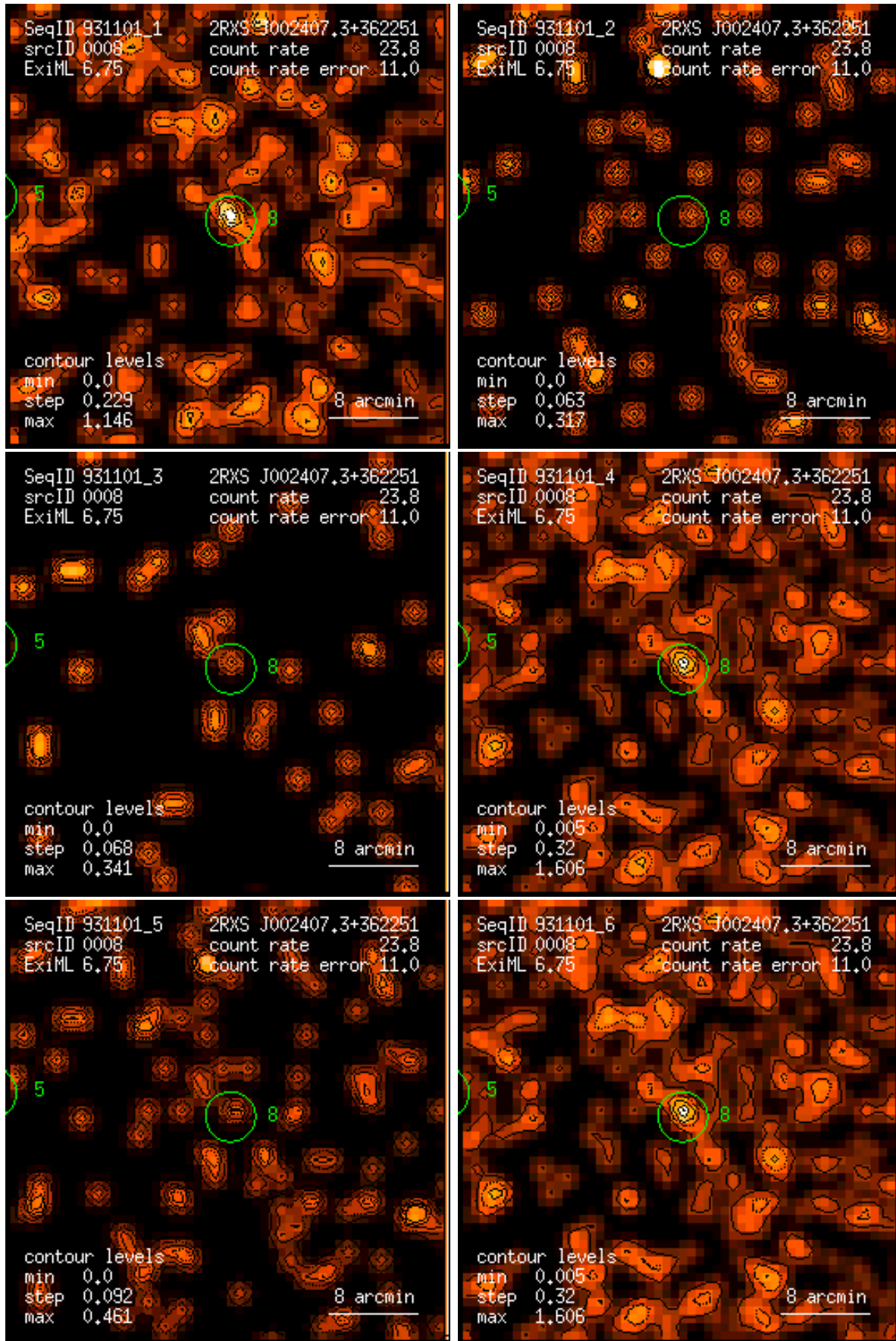
Figure 8: RASS 931101: detection 0008: band rate images, Gaussian filter: (1) PSPC channels 11 – 41, (2) 52 – 90, (3) 91 – 201, (4) 11 – 235, (5) 52 – 201, (6) 11 – 201. Broad band rates in counts/ks. Band rate contour levels in counts/ks/arcmin 2 .
