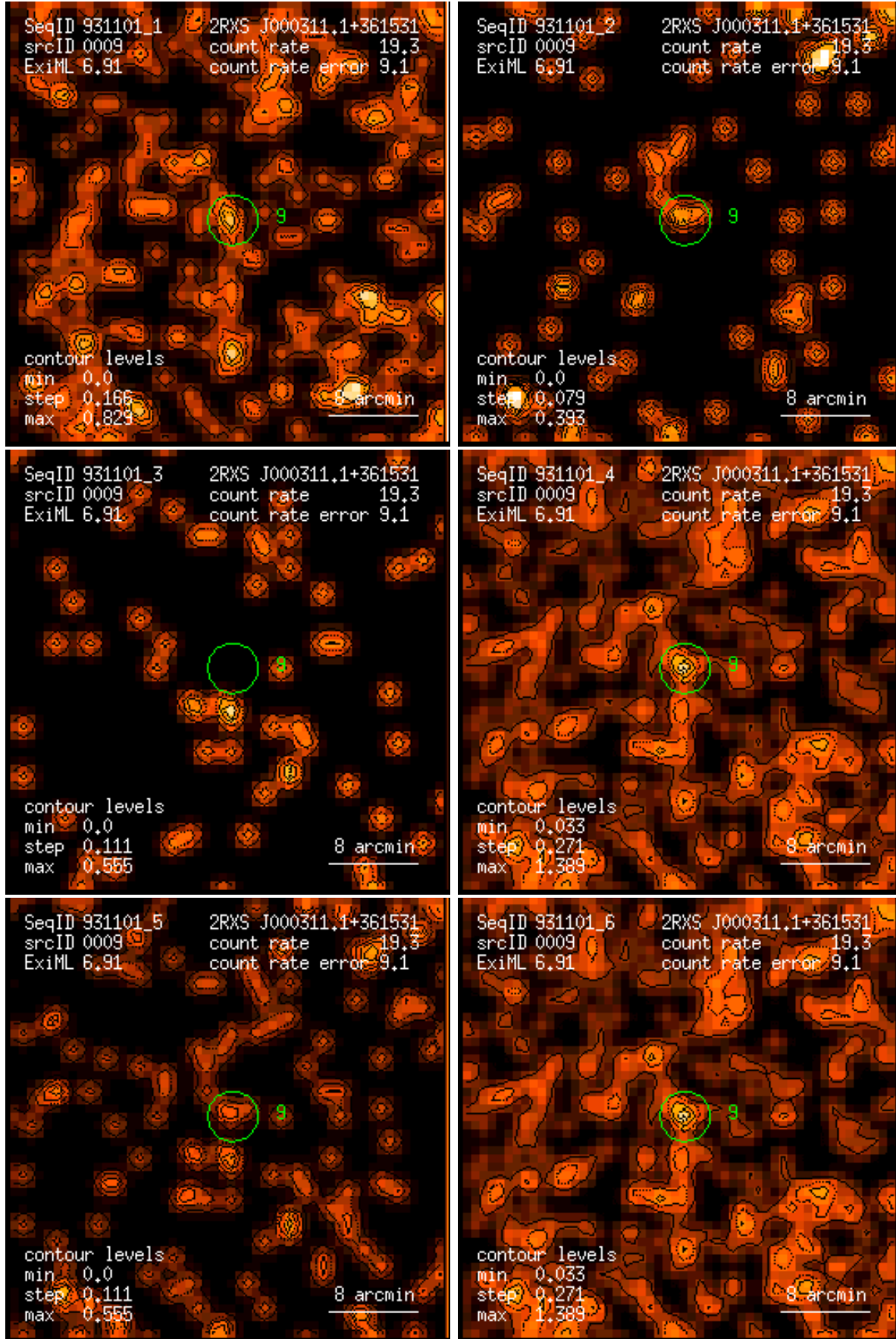
Figure 9: RASS 931101: detection 0009: band rate images, Gaussian filter: (1) PSPC channels 11 – 41, (2) 52 – 90, (3) 91 – 201, (4) 11 – 235, (5) 52 – 201, (6) 11 – 201. Broad band rates in counts/ks. Band rate contour levels in counts/ks/arcmin 2 .
