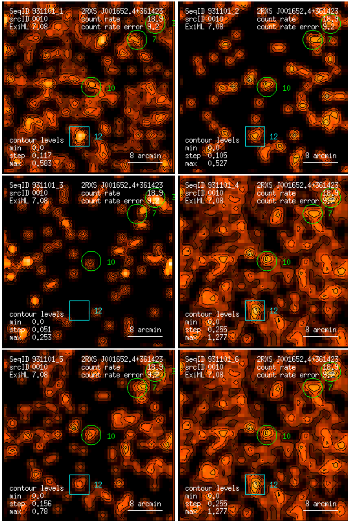
Figure 10: RASS 931101: detection 0010: band rate images, Gaussian filter: (1) PSPC channels 11 – 41, (2) 52 – 90, (3) 91 – 201, (4) 11 – 235, (5) 52 – 201, (6) 11 – 201. Broad band rates in counts/ks. Band rate contour levels in counts/ks/arcmin 2 .
