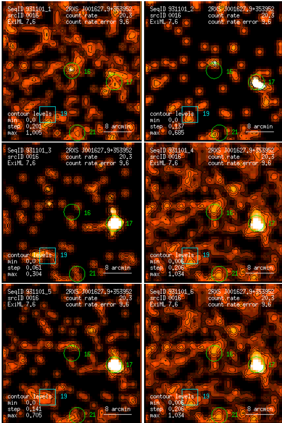
Figure 16: RASS 931101: detection 0016: band rate images, Gaussian filter: (1) PSPP channels 11 – 41, (2) 52 – 90, (3) 91 – 201, (4) 11 – 235, (5) 52 – 201, (6) 11 – 201. Broad band rates in counts/ks. Band rate contour levels in counts/ks/arcmin 2 .
