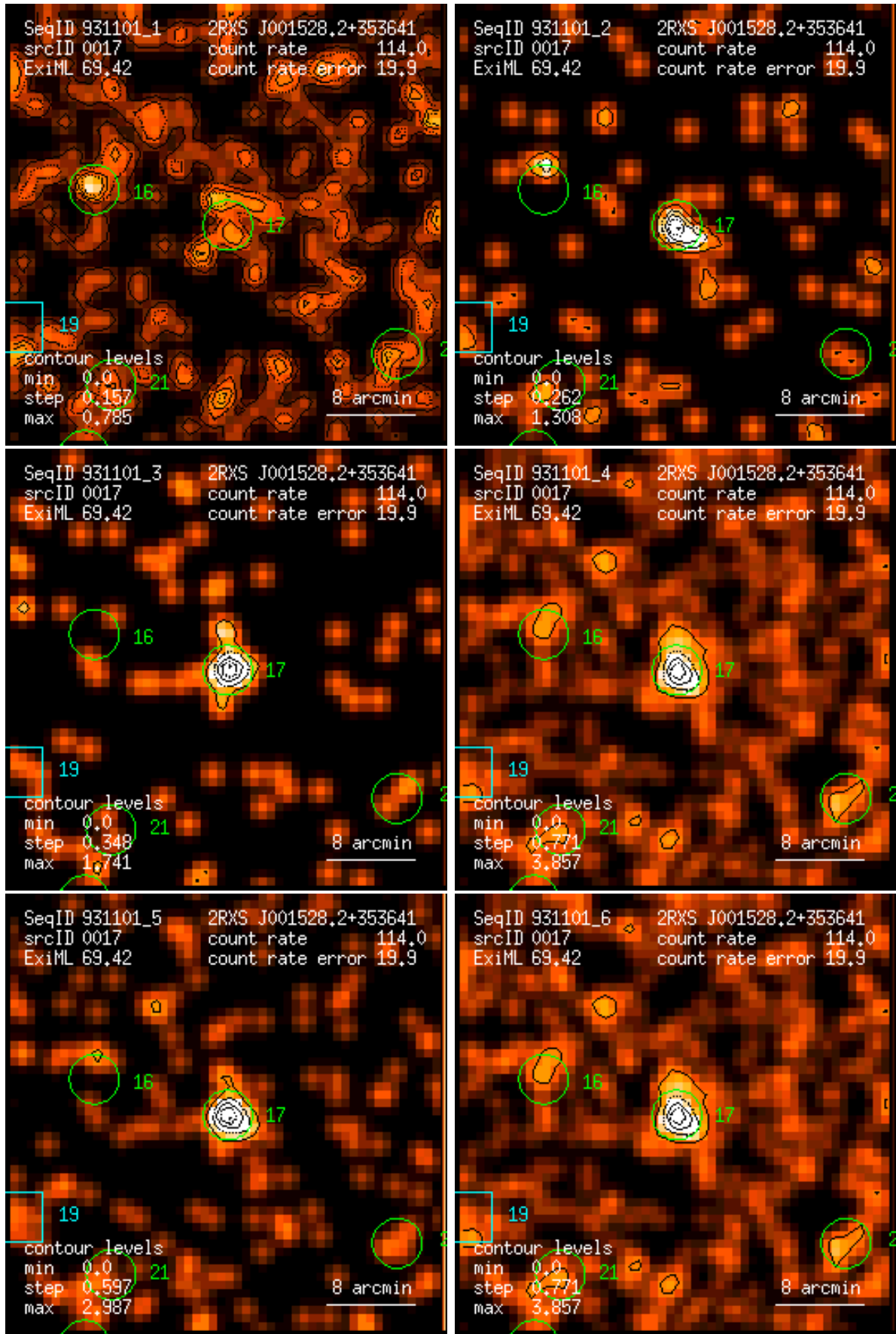
Figure 17: RASS 931101: detection 0017: band rate images, Gaussian filter: (1) PSPC channels 11 – 41, (2) 52 – 90, (3) 91 – 201, (4) 11 – 235, (5) 52 – 201, (6) 11 – 201. Broad band rates in counts/ks. Band rate contour levels in counts/ks/arcmin 2 .
