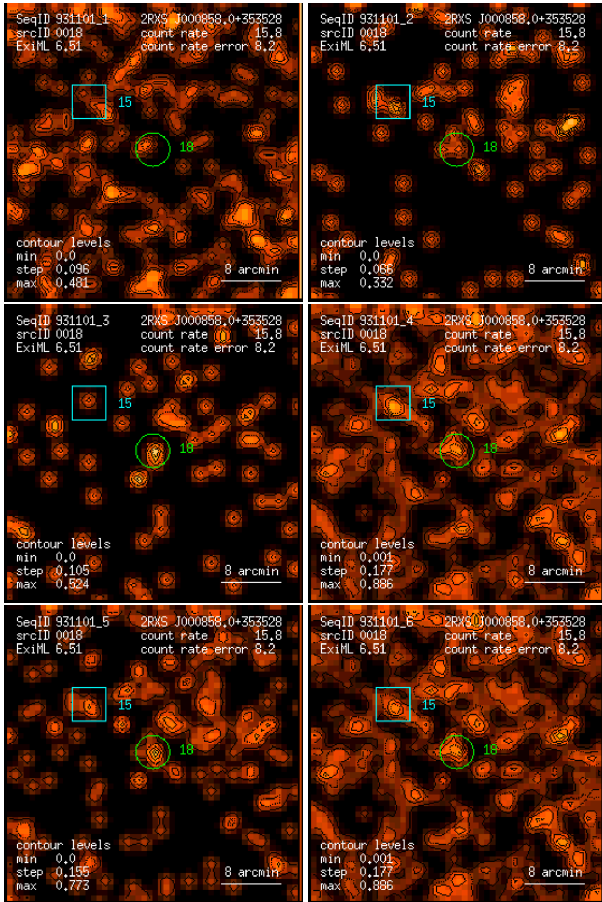
Figure 18: RASS 931101: detection 0018: band rate images, Gaussian filter: (1) PSPC channels 11 – 41, (2) 52 – 90, (3) 91 – 201, (4) 11 – 235, (5) 52 – 201, (6) 11 – 201. Broad band rates in counts/ks. Band rate contour levels in counts/ks/arcmin 2 .
