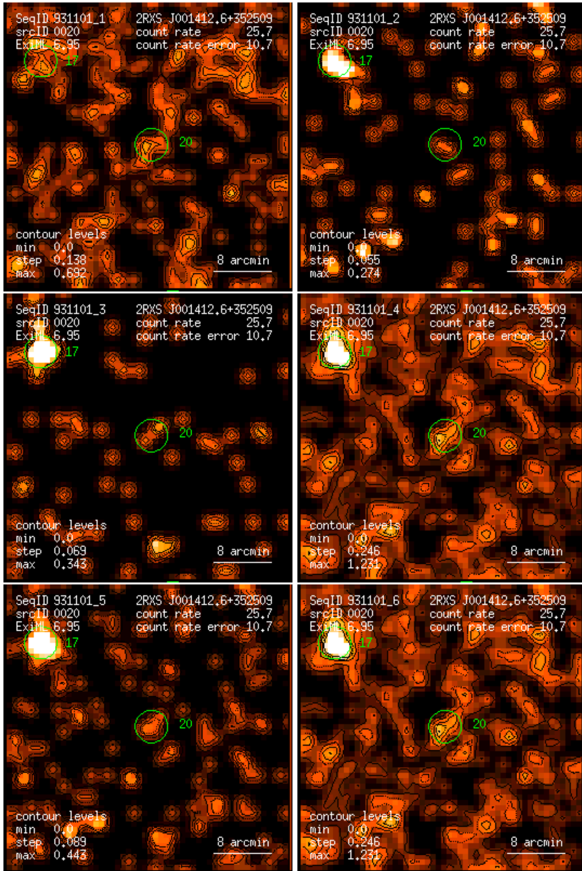
Figure 20: RASS 931101: detection 0020: band rate images, Gaussian filter: (1) PSPC channels 11 – 41, (2) 52 – 90, (3) 91 – 201, (4) 11 – 235, (5) 52 – 201, (6) 11 – 201. Broad band rates in counts/ks. Band rate contour levels in counts/ks/arcmin 2 .
