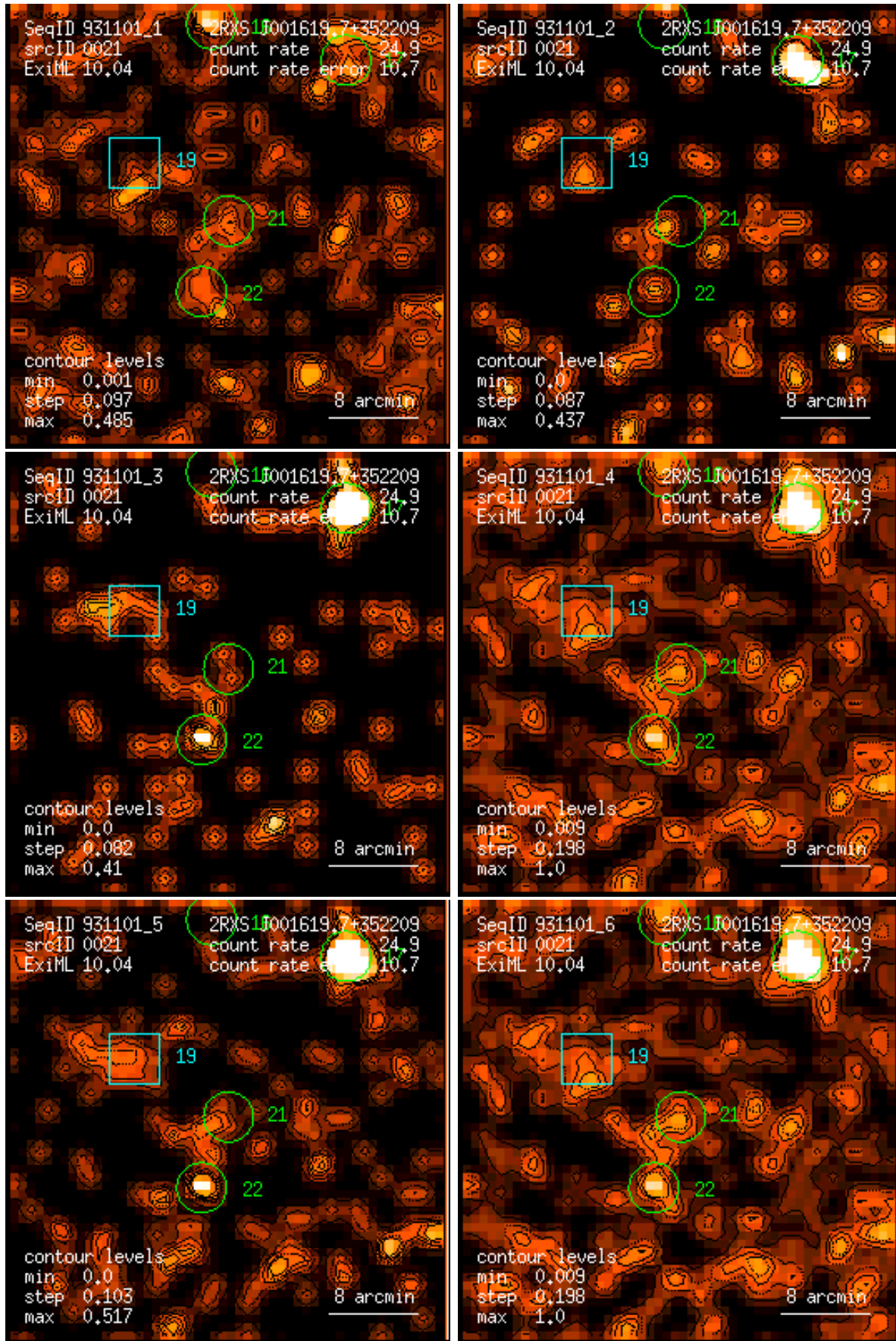
Figure 21: RASS 931101: detection 0021: band rate images, Gaussian filter: (1) PSPC channels 11 – 41, (2) 52 – 90, (3) 91 – 201, (4) 11 – 235, (5) 52 – 201, (6) 11 – 201. Broad band rates in counts/ks. Band rate contour levels in counts/ks/arcmin 2 .
