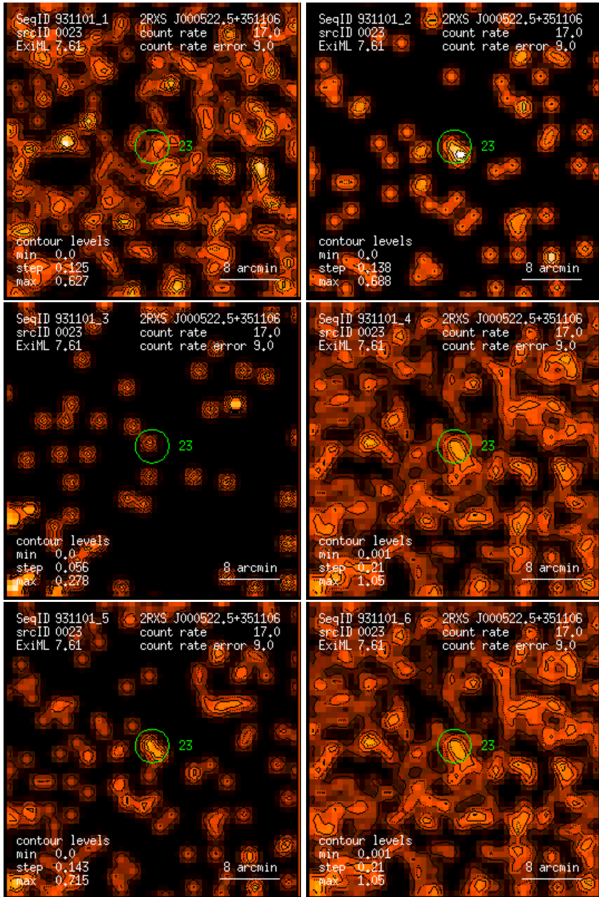
Figure 23: RASS 931101: detection 0023: band rate images, Gaussian filter: (1) PSPC channels 11 – 41, (2) 52 – 90, (3) 91 – 201, (4) 11 – 235, (5) 52 – 201, (6) 11 – 201. Broad band rates in counts/ks. Band rate contour levels in counts/ks/arcmin 2 .
