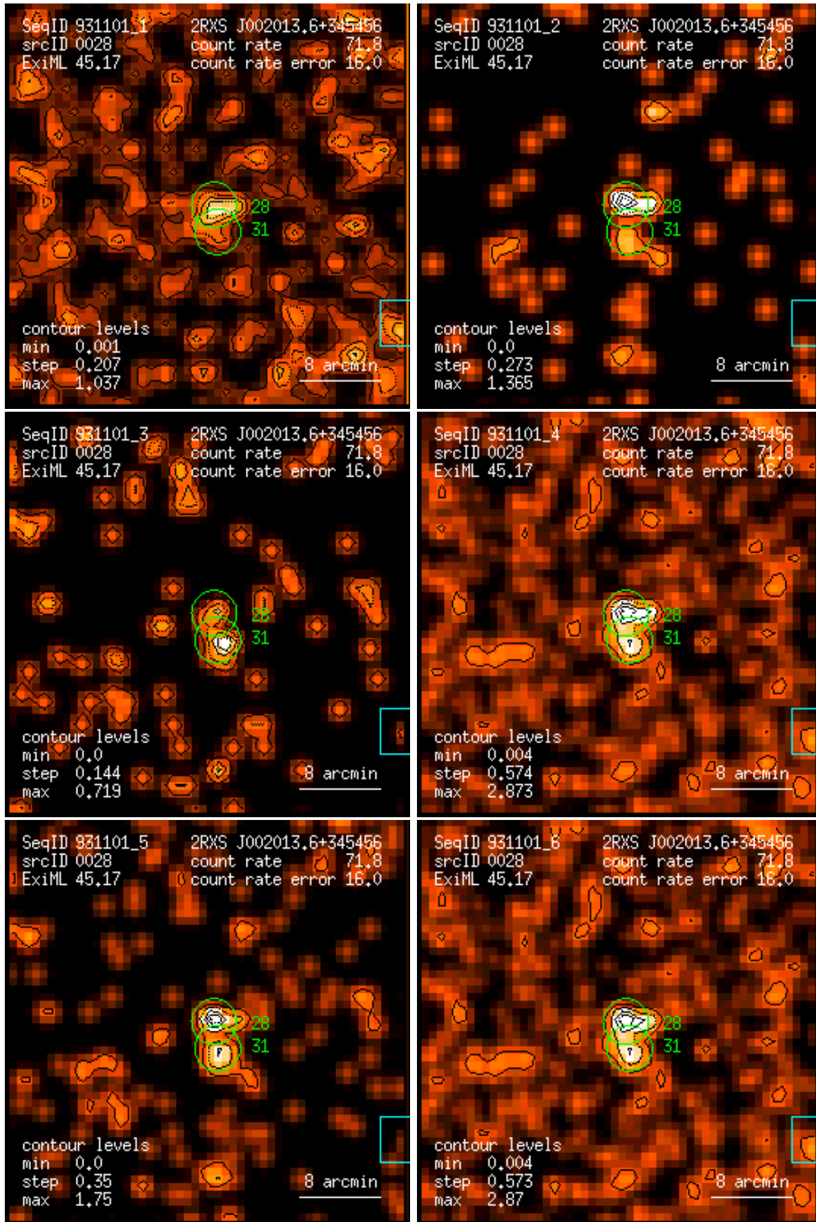
Figure 28: RASS 931101: detection 0028: band rate images, Gaussian filter: (1) PSPC channels 11 – 41, (2) 52 – 90, (3) 91 – 201, (4) 11 – 235, (5) 52 – 201, (6) 11 – 201. Broad band rates in counts/ks. Band rate contour levels in counts/ks/arcmin 2 .
