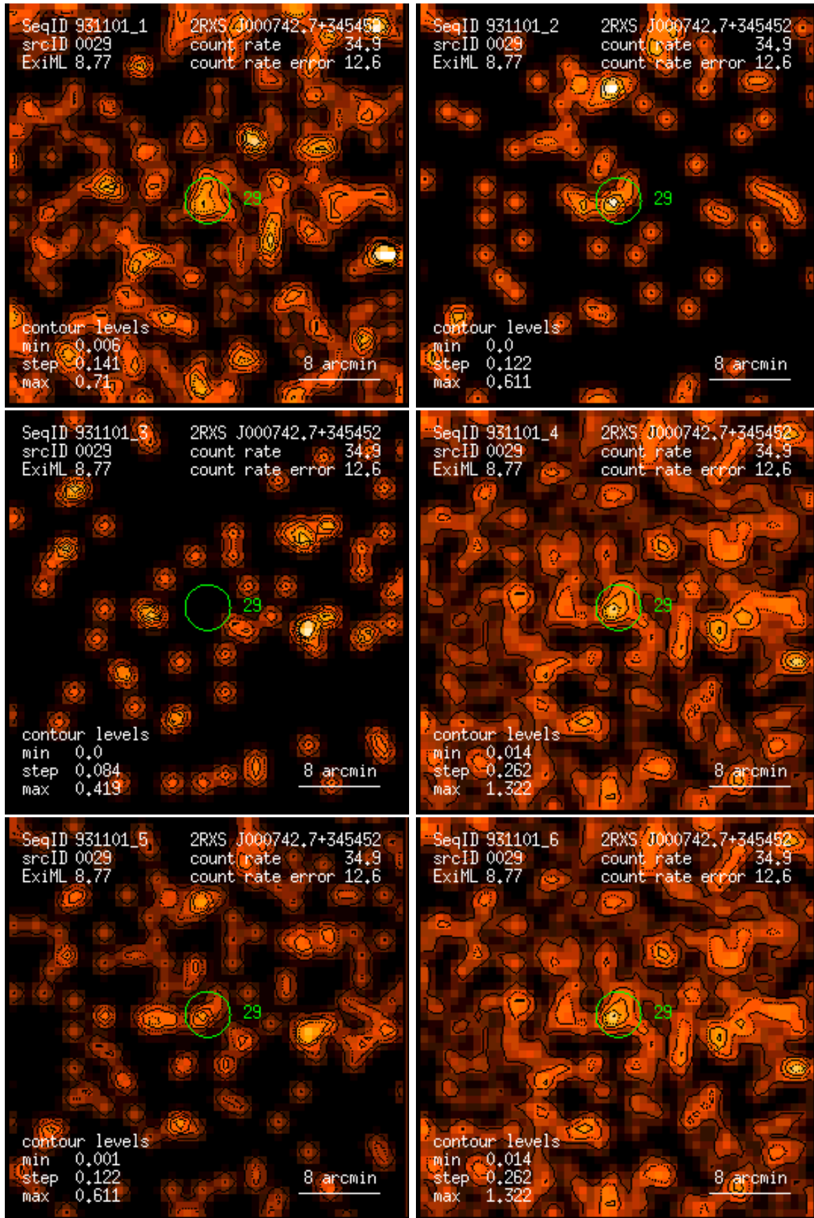
Figure 29: RASS 931101: detection 0029: band rate images, Gaussian filter: (1) PSPC channels 11 – 41, (2) 52 – 90, (3) 91 – 201, (4) 11 – 235, (5) 52 – 201, (6) 11 – 201. Broad band rates in counts/ks. Band rate contour levels in counts/ks/arcmin 2 .
