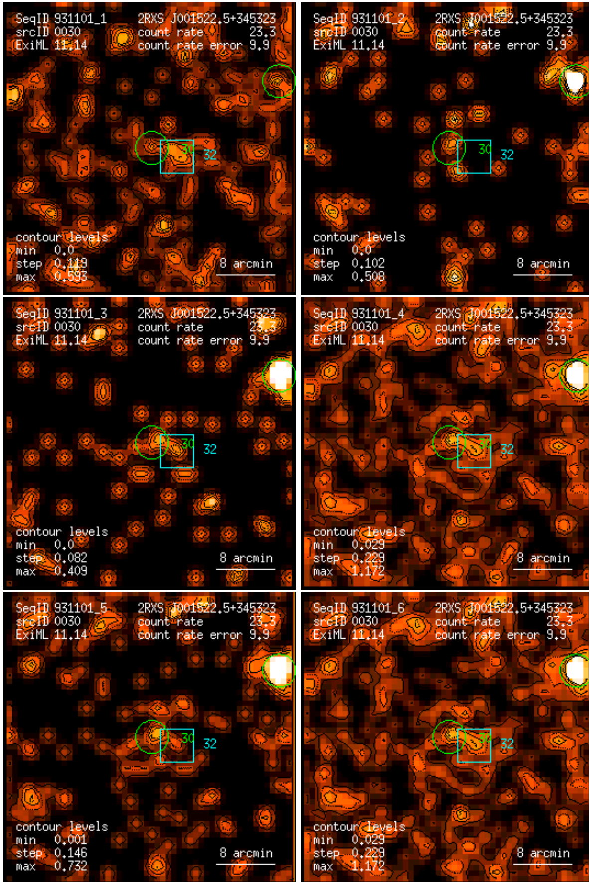
Figure 30: RASS 931101: detection 0030: band rate images, Gaussian filter: (1) PSPC channels 11 – 41, (2) 52 – 90, (3) 91 – 201, (4) 11 – 235, (5) 52 – 201, (6) 11 – 201. Broad band rates in counts/ks. Band rate contour levels in counts/ks/arcmin 2 .
