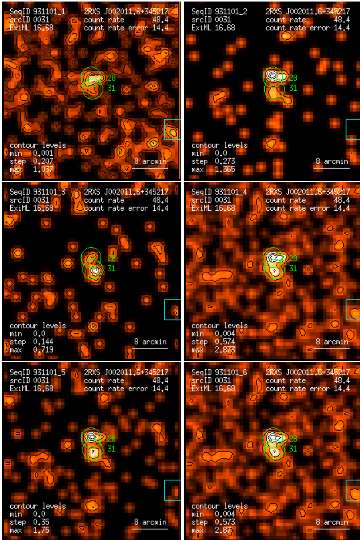
Figure 31: RASS 931101: detection 0031: band rate images, Gaussian filter: (1) PSPC channels 11 – 41, (2) 52 – 90, (3) 91 – 201, (4) 11 – 235, (5) 52 – 201, (6) 11 – 201. Broad band rates in counts/ks. Band rate contour levels in counts/ks/arcmin 2 .
