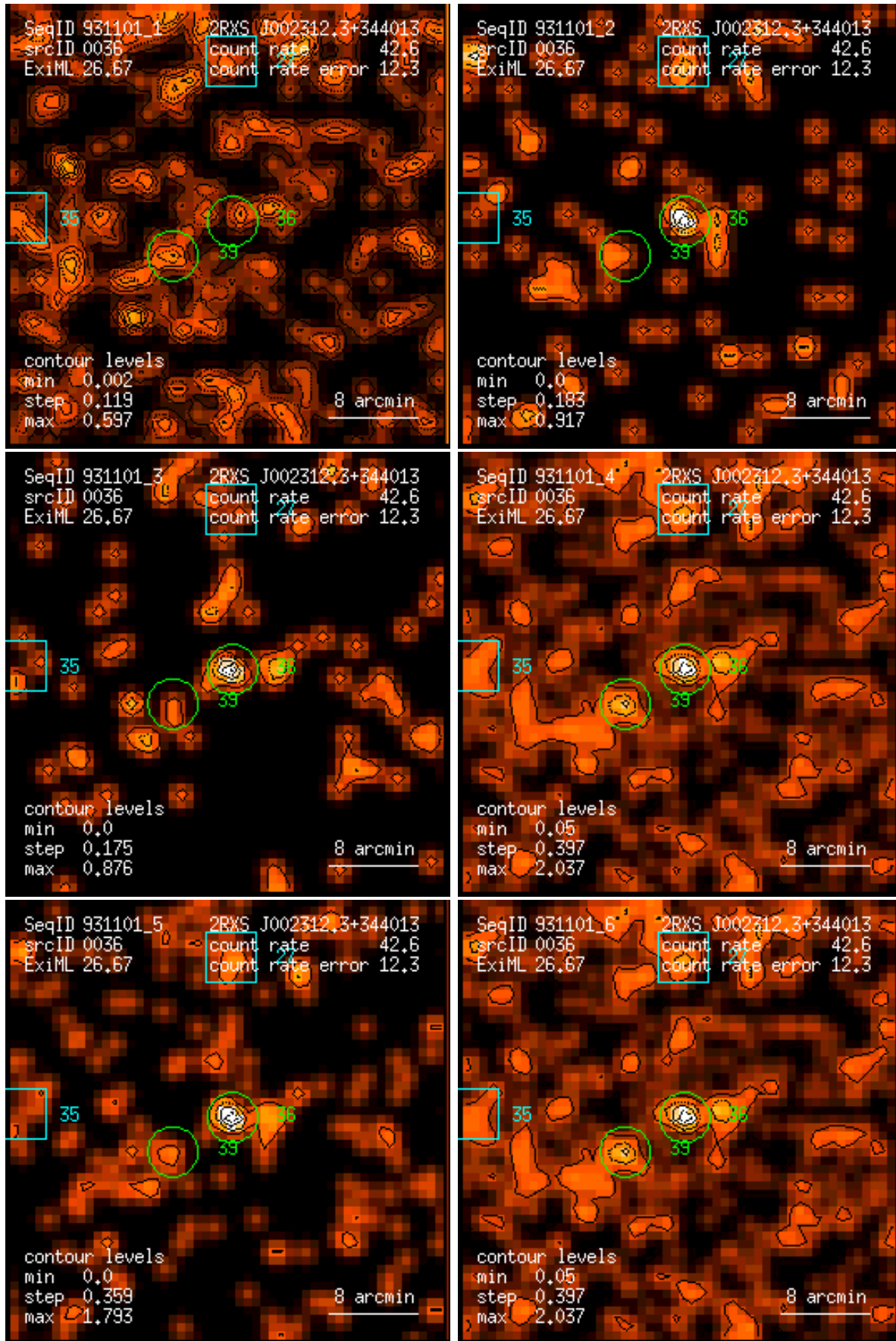
Figure 36: RASS 931101: detection 0036: band rate images, Gaussian filter: (1) PSPC channels 11 – 41, (2) 52 – 90, (3) 91 – 201, (4) 11 – 235, (5) 52 – 201, (6) 11 – 201. Broad band rates in counts/ks. Band rate contour levels in counts/ks/arcmin 2 .
