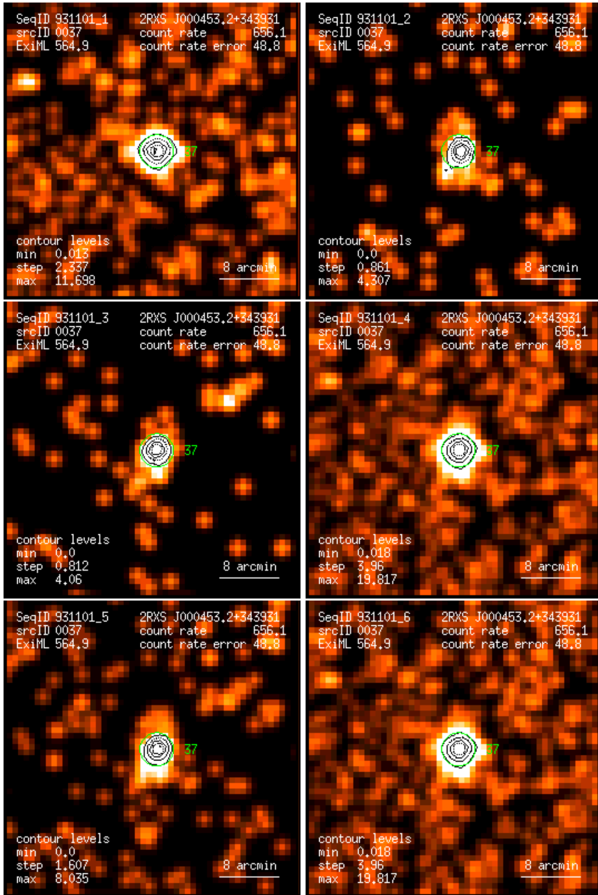
Figure 37: RASS 931101: detection 0037: band rate images, Gaussian filter: (1) PSPC channels 11 – 41, (2) 52 – 90, (3) 91 – 201, (4) 11 – 235, (5) 52 – 201, (6) 11 – 201. Broad band rates in counts/ks. Band rate contour levels in counts/ks/arcmin 2 .
