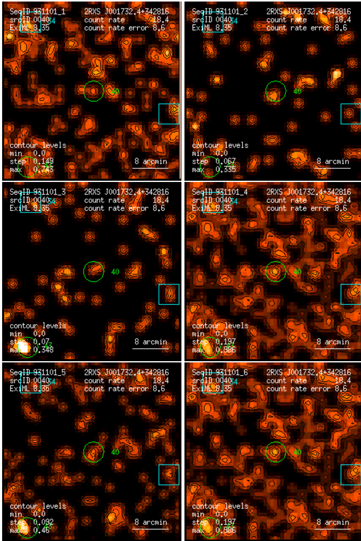
Figure 40: RASS 931101: detection 0040: band rate images, Gaussian filter: (1) PSPC channels 11 – 41, (2) 52 – 90, (3) 91 – 201, (4) 11 – 235, (5) 52 – 201, (6) 11 – 201. Broad band rates in counts/ks. Band rate contour levels in counts/ks/arcmin 2 .
