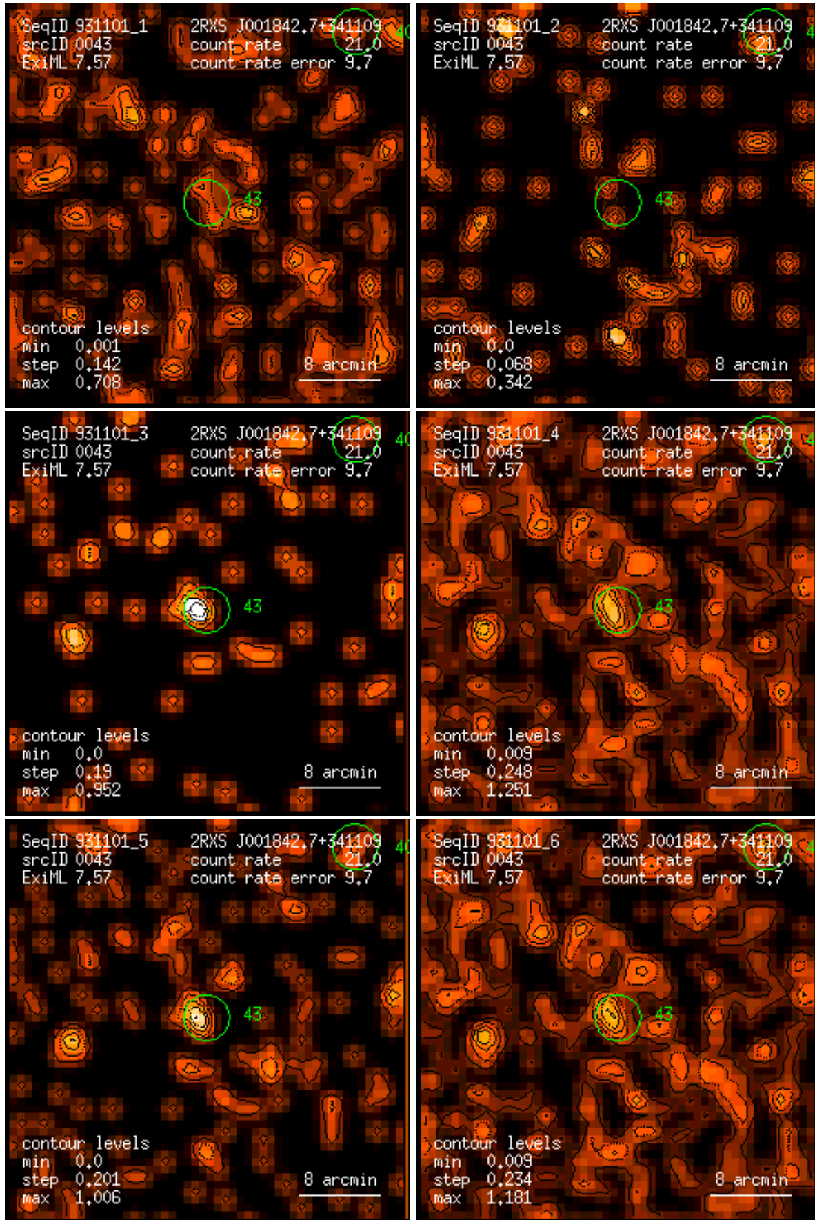
Figure 43: RASS 931101: detection 0043: band rate images, Gaussian filter: (1) PSPC channels 11 – 41, (2) 52 – 90, (3) 91 – 201, (4) 11 – 235, (5) 52 – 201, (6) 11 – 201. Broad band rates in counts/ks. Band rate contour levels in counts/ks/arcmin 2 .
