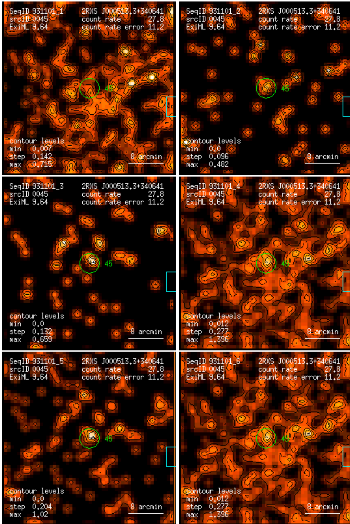
Figure 45: RASS 931101: detection 0045: band rate images, Gaussian filter: (1) PSPC channels 11 – 41, (2) 52 – 90, (3) 91 – 201, (4) 11 – 235, (5) 52 – 201, (6) 11 – 201. Broad band rates in counts/ks. Band rate contour levels in counts/ks/arcmin 2 .
