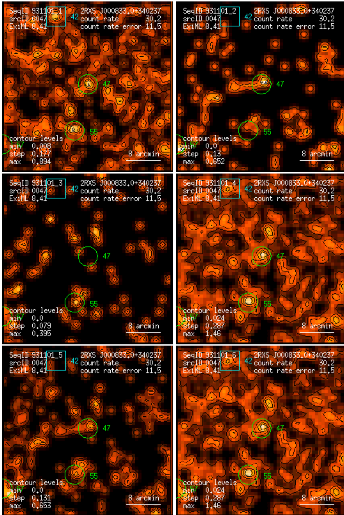
Figure 47: RASS 931101: detection 0047: band rate images, Gaussian filter: (1) PSPC channels 11 – 41, (2) 52 – 90, (3) 91 – 201, (4) 11 – 235, (5) 52 – 201, (6) 11 – 201. Broad band rates in counts/ks. Band rate contour levels in counts/ks/arcmin 2 .
