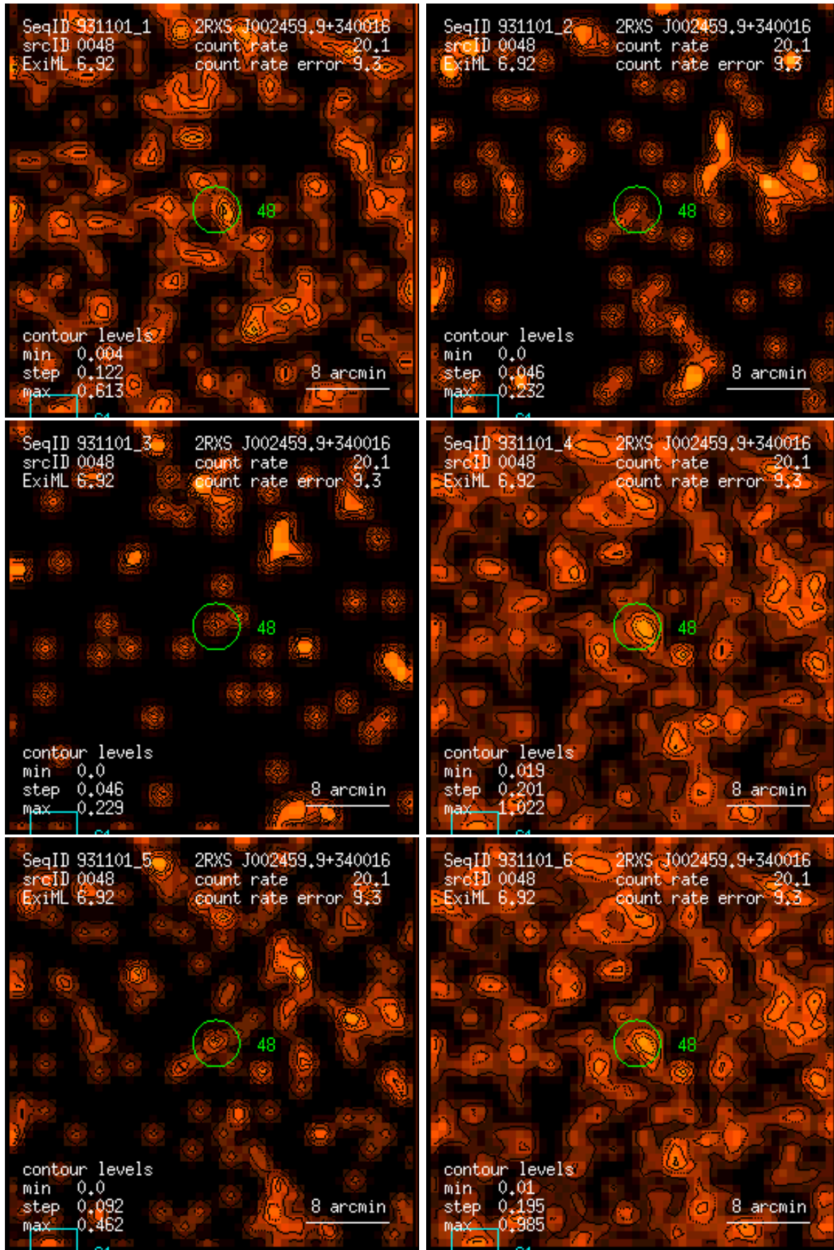
Figure 48: RASS 931101: detection 0048: band rate images, Gaussian filter: (1) PSPC channels 11 – 41, (2) 52 – 90, (3) 91 – 201, (4) 11 – 235, (5) 52 – 201, (6) 11 – 201. Broad band rates in counts/ks. Band rate contour levels in counts/ks/arcmin 2 .
