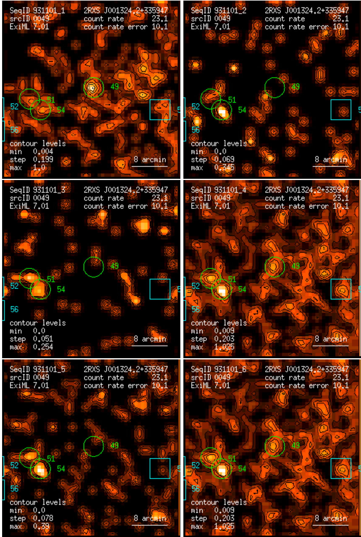
Figure 49: RASS 931101: detection 0049: band rate images, Gaussian filter: (1) PSPC channels 11 – 41, (2) 52 – 90, (3) 91 – 201, (4) 11 – 235, (5) 52 – 201, (6) 11 – 201. Broad band rates in counts/ks. Band rate contour levels in counts/ks/arcmin 2 .
