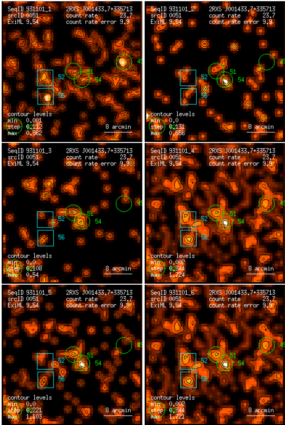
Figure 51: RASS 931101: detection 0051: band rate images, Gaussian filter: (1) PSPC channels 11 – 41, (2) 52 – 90, (3) 91 – 201, (4) 11 – 235, (5) 52 – 201, (6) 11 – 201. Broad band rates in counts/ks. Band rate contour levels in counts/ks/arcmin 2 .
