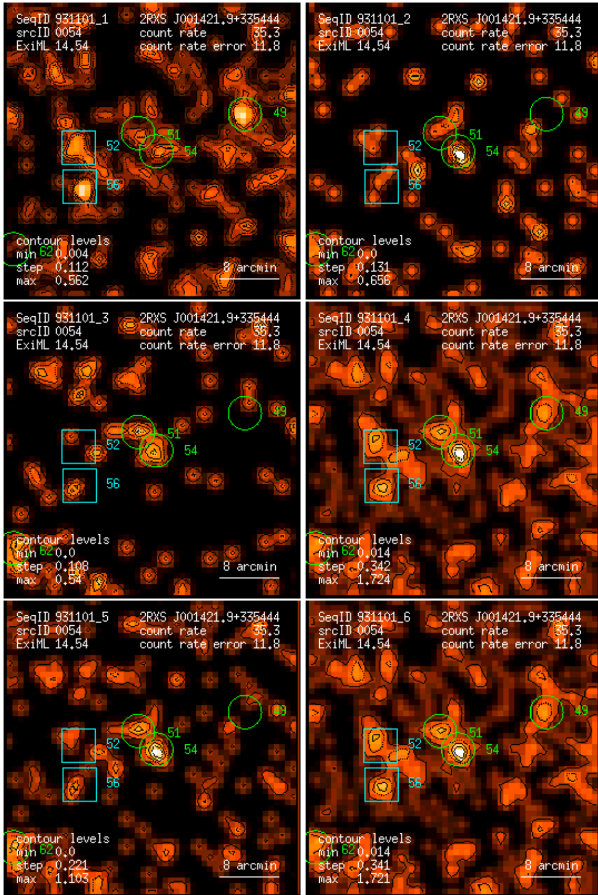
Figure 54: RASS 931101: detection 0054: band rate images, Gaussian filter: (1) PSPC channels 11 – 41, (2) 52 – 90, (3) 91 – 201, (4) 11 – 235, (5) 52 – 201, (6) 11 – 201. Broad band rates in counts/ks. Band rate contour levels in counts/ks/arcmin 2 .
