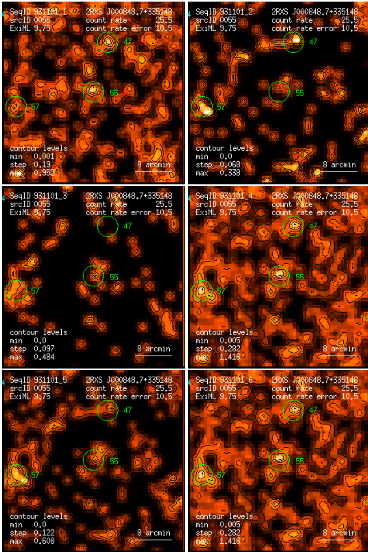
Figure 55: RASS 931101: detection 0055: band rate images, Gaussian filter: (1) PSPC channels 11 – 41, (2) 52 – 90, (3) 91 – 201, (4) 11 – 235, (5) 52 – 201, (6) 11 – 201. Broad band rates in counts/ks. Band rate contour levels in counts/ks/arcmin 2 .
