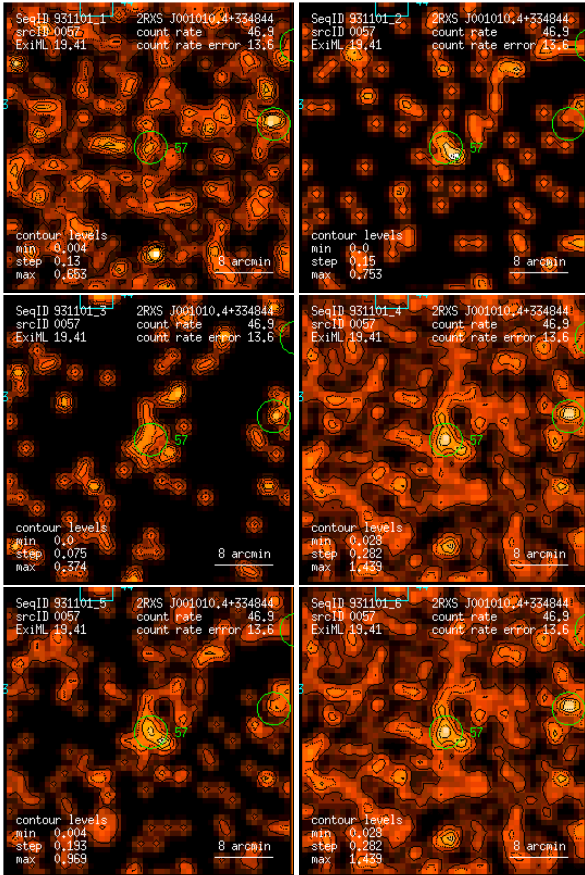
Figure 57: RASS 931101: detection 0057: band rate images, Gaussian filter: (1) PSPC channels 11 – 41, (2) 52 – 90, (3) 91 – 201, (4) 11 – 235, (5) 52 – 201, (6) 11 – 201. Broad band rates in counts/ks. Band rate contour levels in counts/ks/arcmin 2 .
