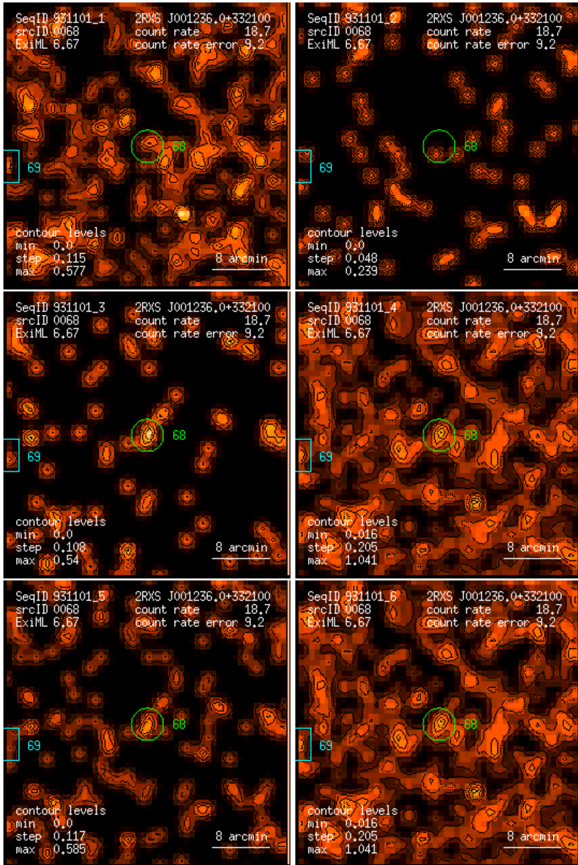
Figure 68: RASS 931101: detection 0068: band rate images, Gaussian filter: (1) PSPC channels 11 – 41, (2) 52 – 90, (3) 91 – 201, (4) 11 – 235, (5) 52 – 201, (6) 11 – 201. Broad band rates in counts/ks. Band rate contour levels in counts/ks/arcmin 2 .
