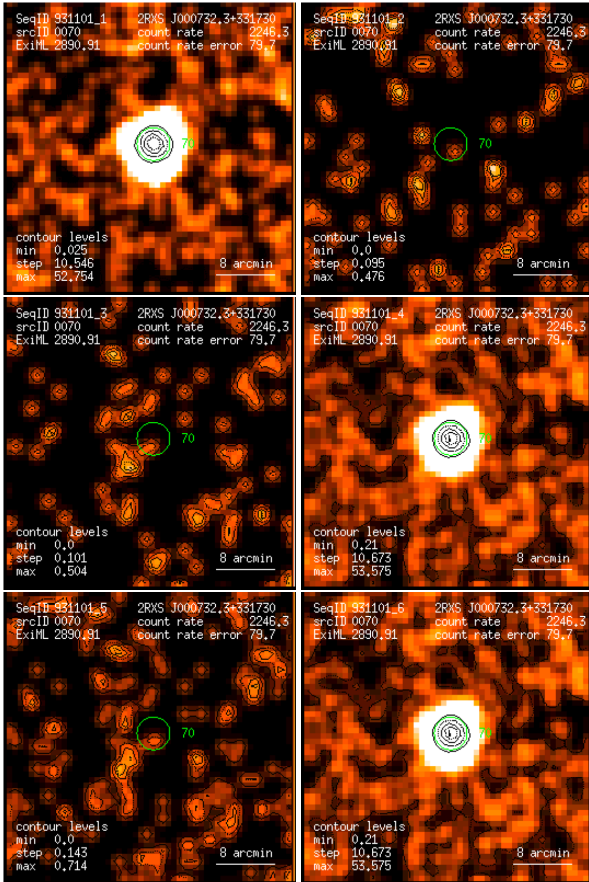
Figure 70: RASS 931101: detection 0070: band rate images, Gaussian filter: (1) PSPC channels 11 – 41, (2) 52 – 90, (3) 91 – 201, (4) 11 – 235, (5) 52 – 201, (6) 11 – 201. Broad band rates in counts/ks. Band rate contour levels in counts/ks/arcmin 2 .
