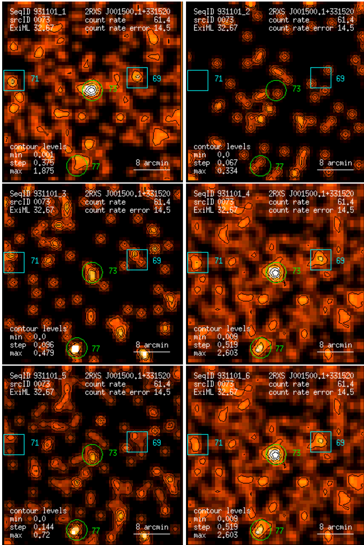
Figure 73: RASS 931101: detection 0073: band rate images, Gaussian filter: (1) PSPC channels 11 – 41, (2) 52 – 90, (3) 91 – 201, (4) 11 – 235, (5) 52 – 201, (6) 11 – 201. Broad band rates in counts/ks. Band rate contour levels in counts/ks/arcmin 2 .
