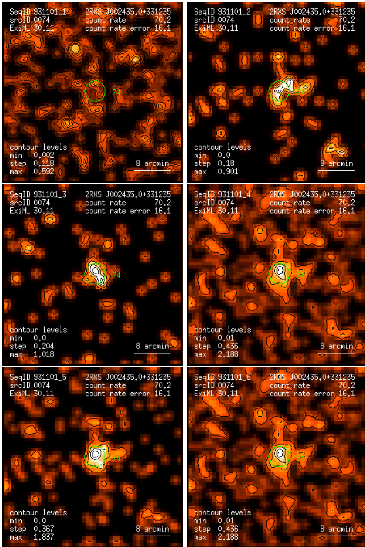
Figure 74: RASS 931101: detection 0074: band rate images, Gaussian filter: (1) PSPC channels 11 – 41, (2) 52 – 90, (3) 91 – 201, (4) 11 – 235, (5) 52 – 201, (6) 11 – 201. Broad band rates in counts/ks. Band rate contour levels in counts/ks/arcmin 2 .
