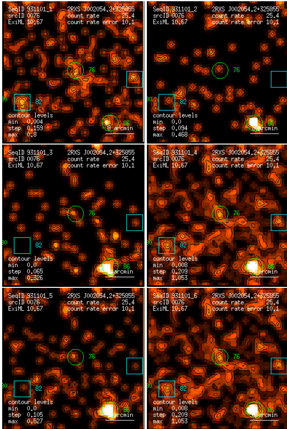
Figure 76: RASS 931101: detection 0076: band rate images, Gaussian filter: (1) PSPC channels 11 – 41, (2) 52 – 90, (3) 91 – 201, (4) 11 – 235, (5) 52 – 201, (6) 11 – 201. Broad band rates in counts/ks. Band rate contour levels in counts/ks/arcmin 2 .
