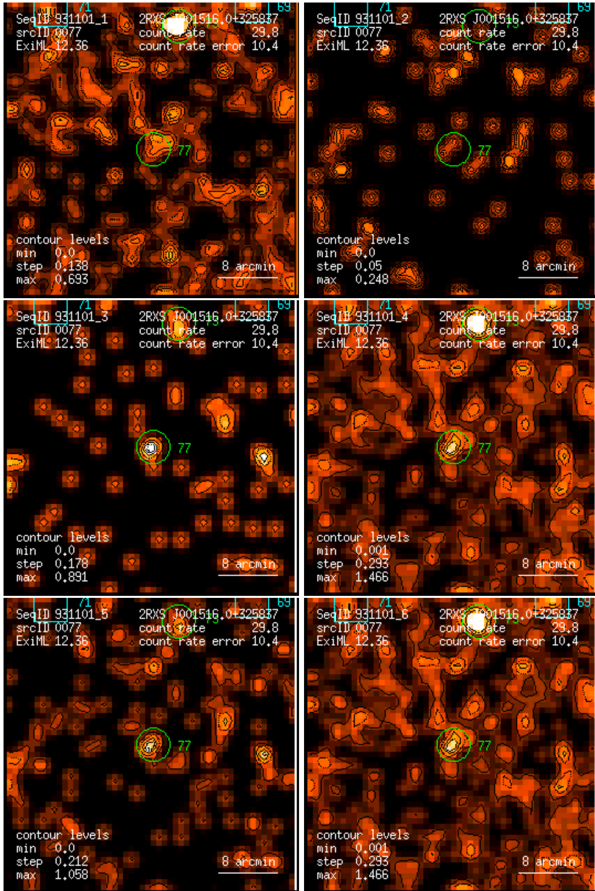
Figure 77: RASS 931101: detection 0077: band rate images, Gaussian filter: (1) PSPC channels 11 – 41, (2) 52 – 90, (3) 91 – 201, (4) 11 – 235, (5) 52 – 201, (6) 11 – 201. Broad band rates in counts/ks. Band rate contour levels in counts/ks/arcmin 2 .
