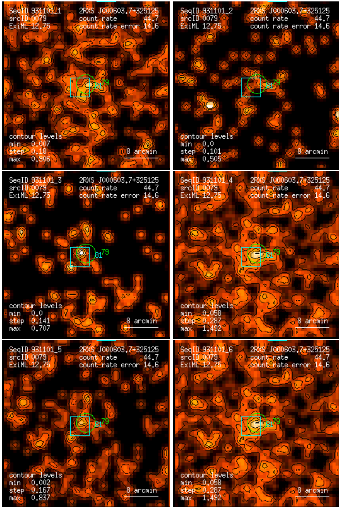
Figure 79: RASS 931101: detection 0079: band rate images, Gaussian filter: (1) PSPC channels 11 – 41, (2) 52 – 90, (3) 91 – 201, (4) 11 – 235, (5) 52 – 201, (6) 11 – 201. Broad band rates in counts/ks. Band rate contour levels in counts/ks/arcmin 2 .
