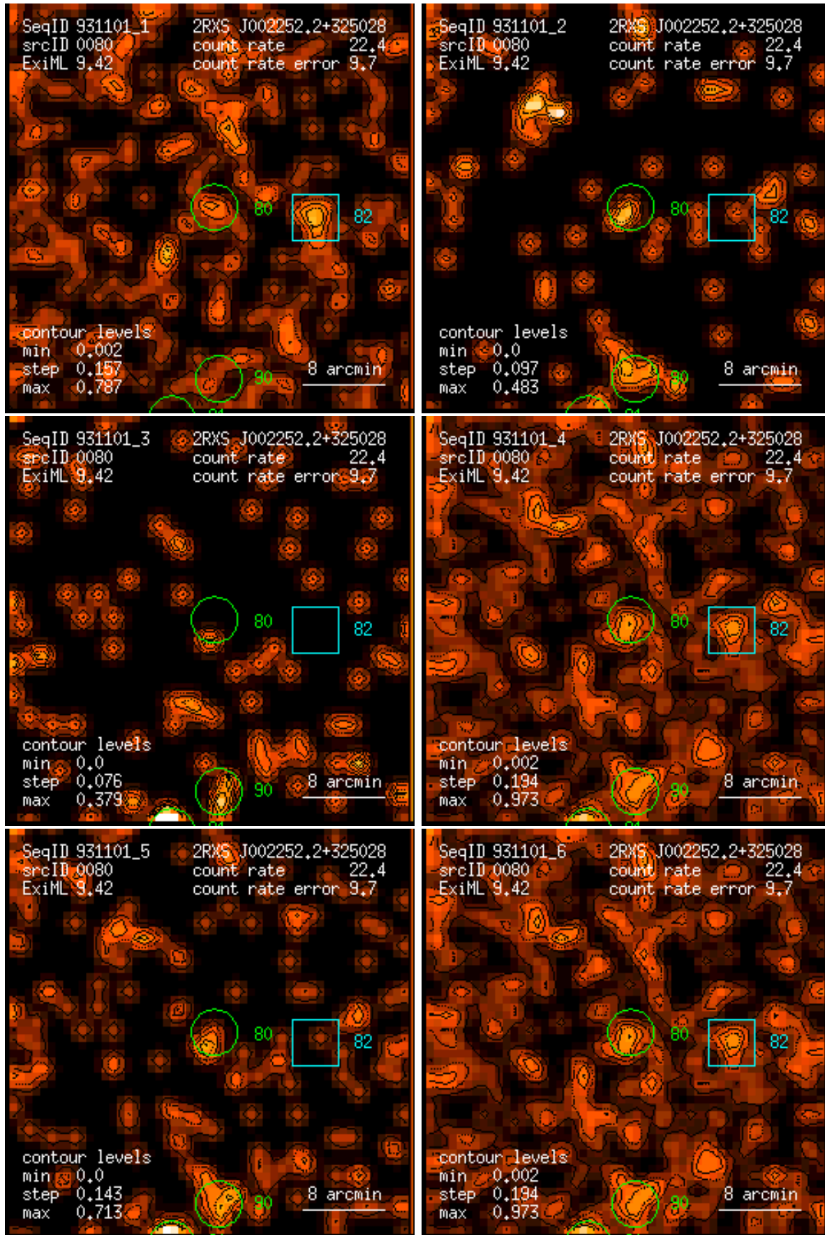
Figure 80: RASS 931101: detection 0080: band rate images, Gaussian filter: (1) PSPC channels 11 – 41, (2) 52 – 90, (3) 91 – 201, (4) 11 – 235, (5) 52 – 201, (6) 11 – 201. Broad band rates in counts/ks. Band rate contour levels in counts/ks/arcmin 2 .
