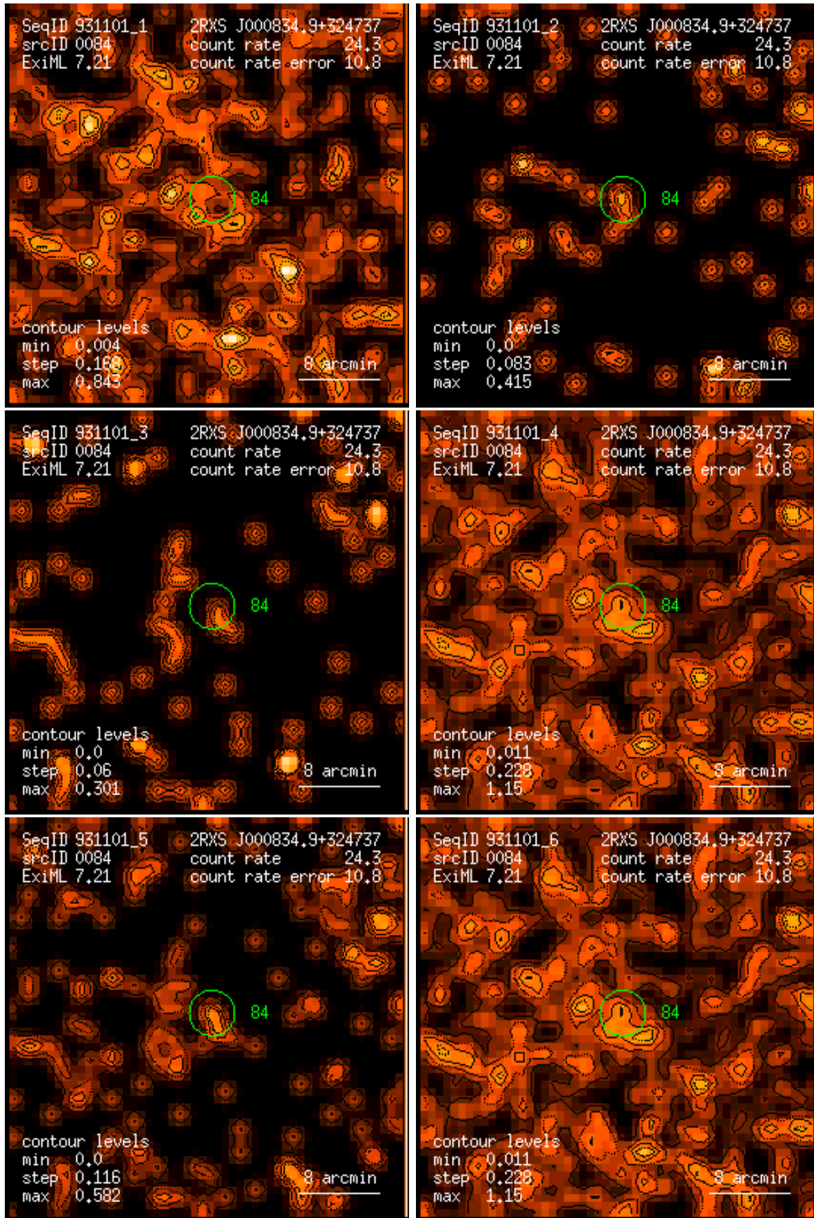
Figure 84: RASS 931101: detection 0084: band rate images, Gaussian filter: (1) PSPC channels 11 – 41, (2) 52 – 90, (3) 91 – 201, (4) 11 – 235, (5) 52 – 201, (6) 11 – 201. Broad band rates in counts/ks. Band rate contour levels in counts/ks/arcmin 2 .
