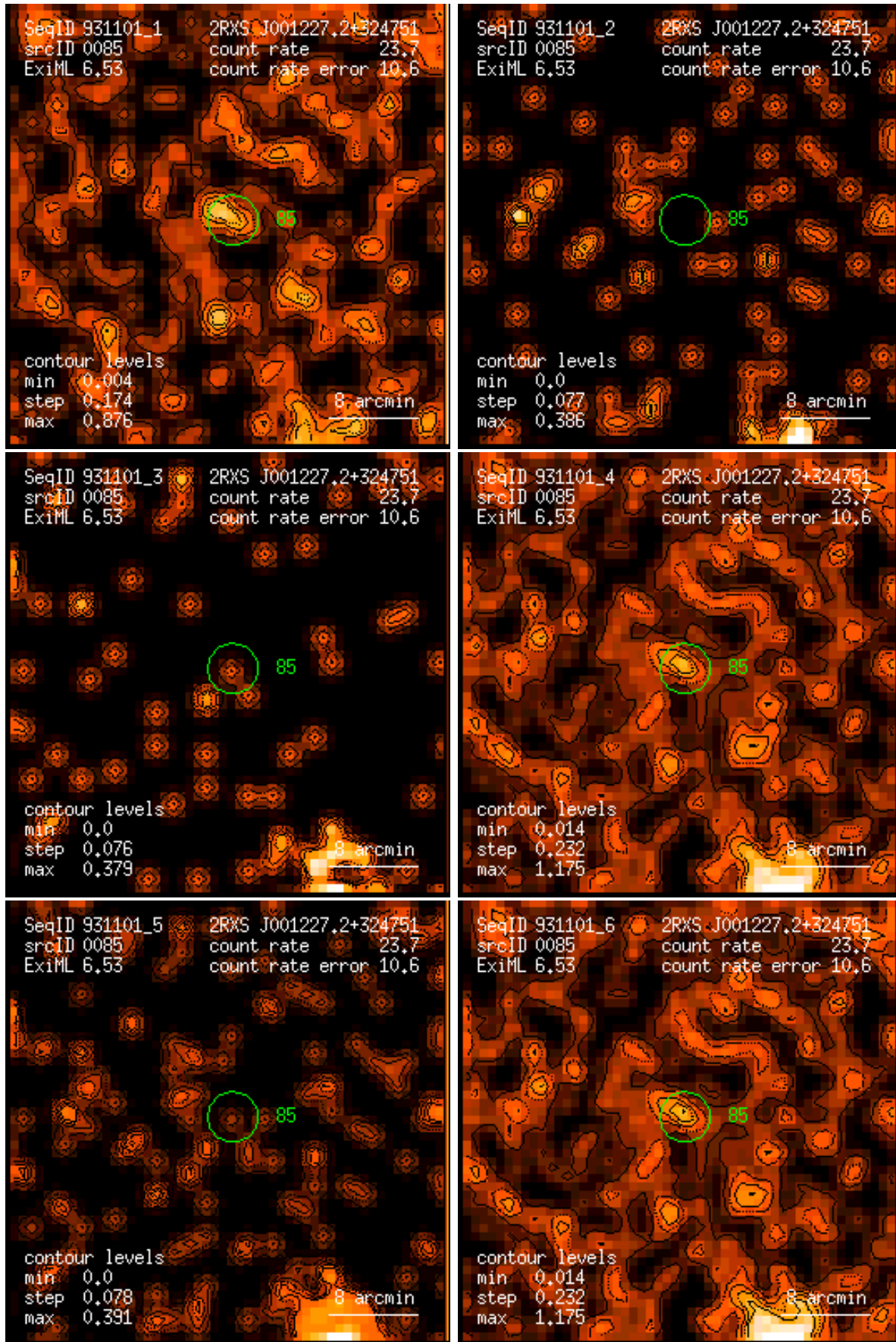
Figure 85: RASS 931101: detection 0085: band rate images, Gaussian filter: (1) PSPC channels 11 – 41, (2) 52 – 90, (3) 91 – 201, (4) 11 – 235, (5) 52 – 201, (6) 11 – 201. Broad band rates in counts/ks. Band rate contour levels in counts/ks/arcmin 2 .
