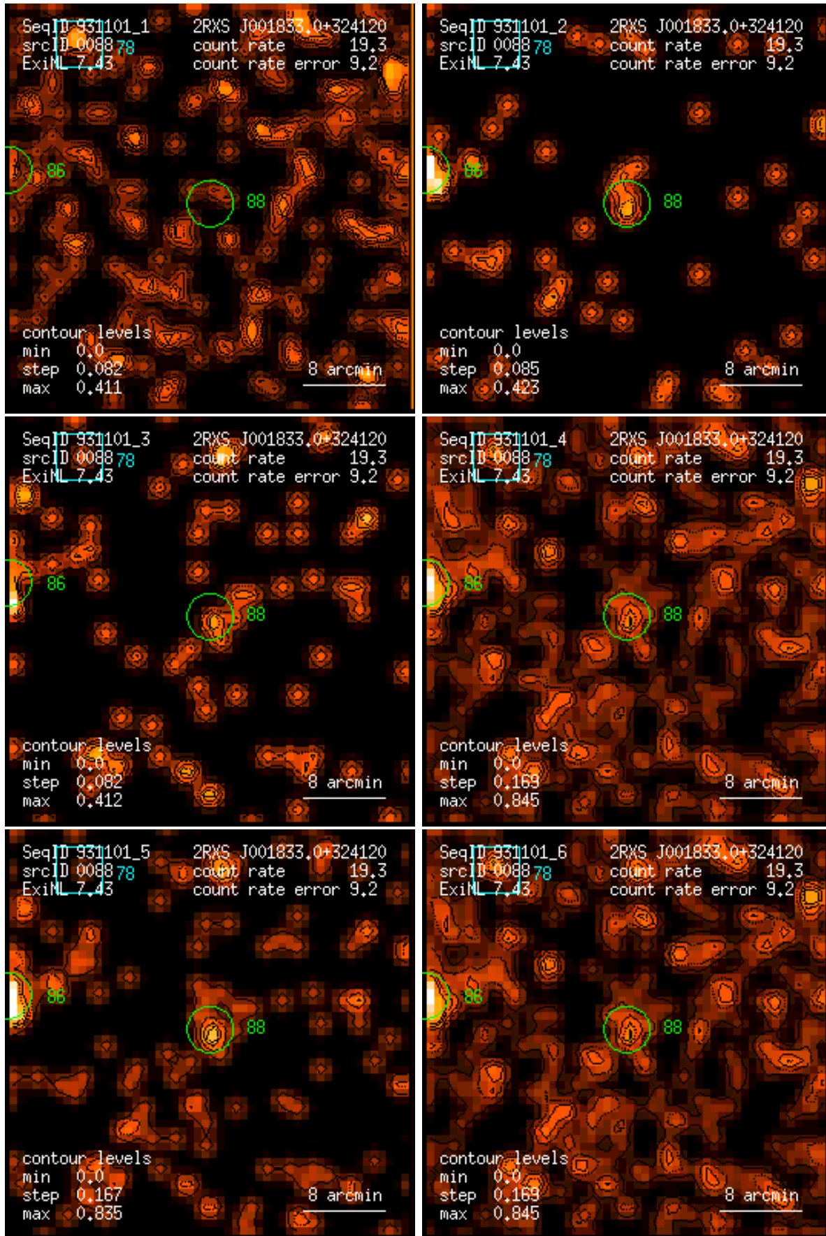
Figure 88: RASS 931101: detection 0088: band rate images, Gaussian filter: (1) PSPC channels 11 – 41, (2) 52 – 90, (3) 91 – 201, (4) 11 – 235, (5) 52 – 201, (6) 11 – 201. Broad band rates in counts/ks. Band rate contour levels in counts/ks/arcmin 2 .
