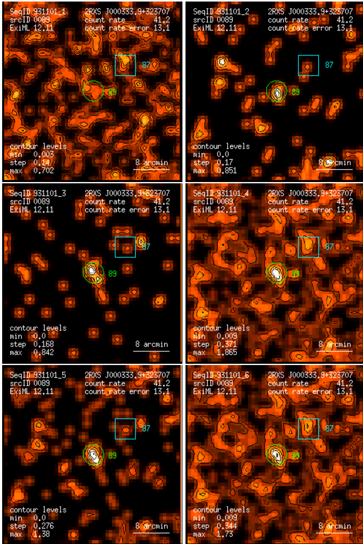
Figure 89: RASS 931101: detection 0089: band rate images, Gaussian filter: (1) PSPC channels 11 – 41, (2) 52 – 90, (3) 91 – 201, (4) 11 – 235, (5) 52 – 201, (6) 11 – 201. Broad band rates in counts/ks. Band rate contour levels in counts/ks/arcmin 2 .
