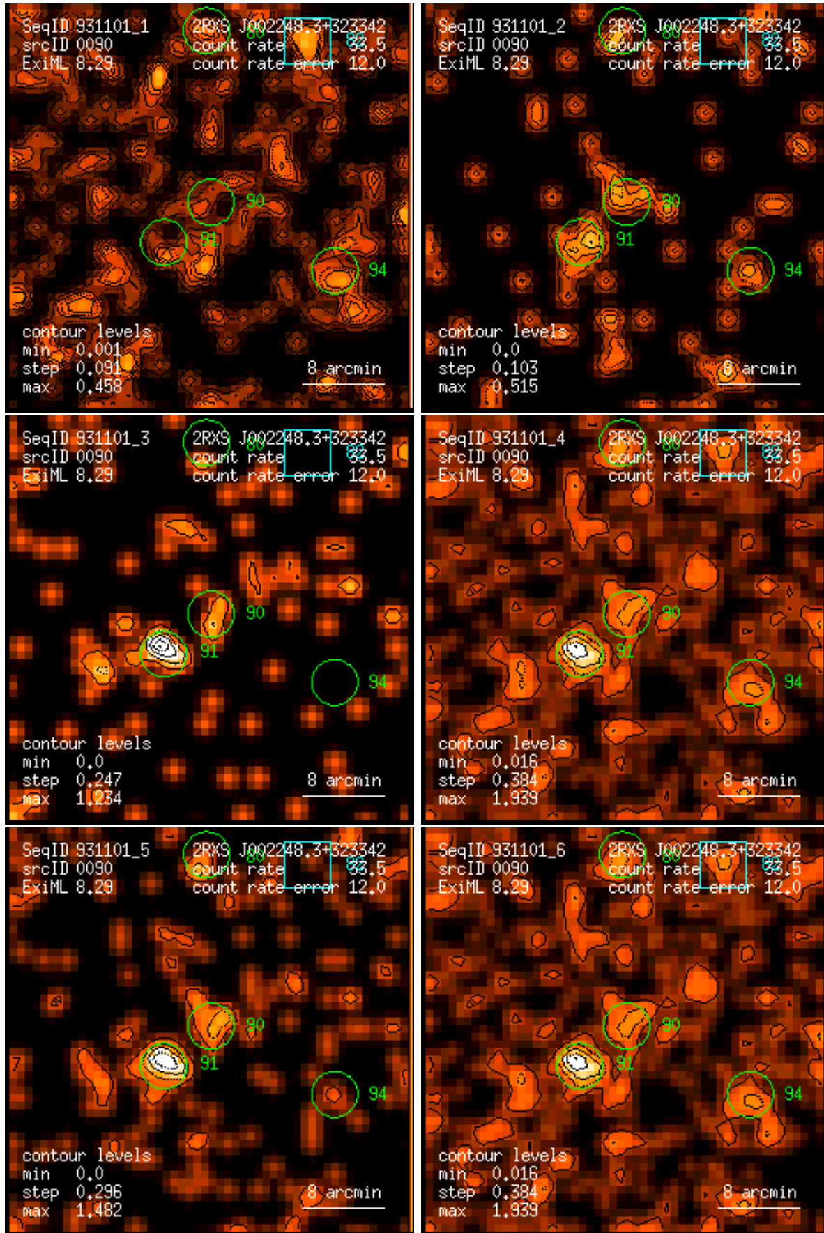
Figure 90: RASS 931101: detection 0090: band rate images, Gaussian filter: (1) PSPC channels 11 – 41, (2) 52 – 90, (3) 91 – 201, (4) 11 – 235, (5) 52 – 201, (6) 11 – 201. Broad band rates in counts/ks. Band rate contour levels in counts/ks/arcmin 2 .
