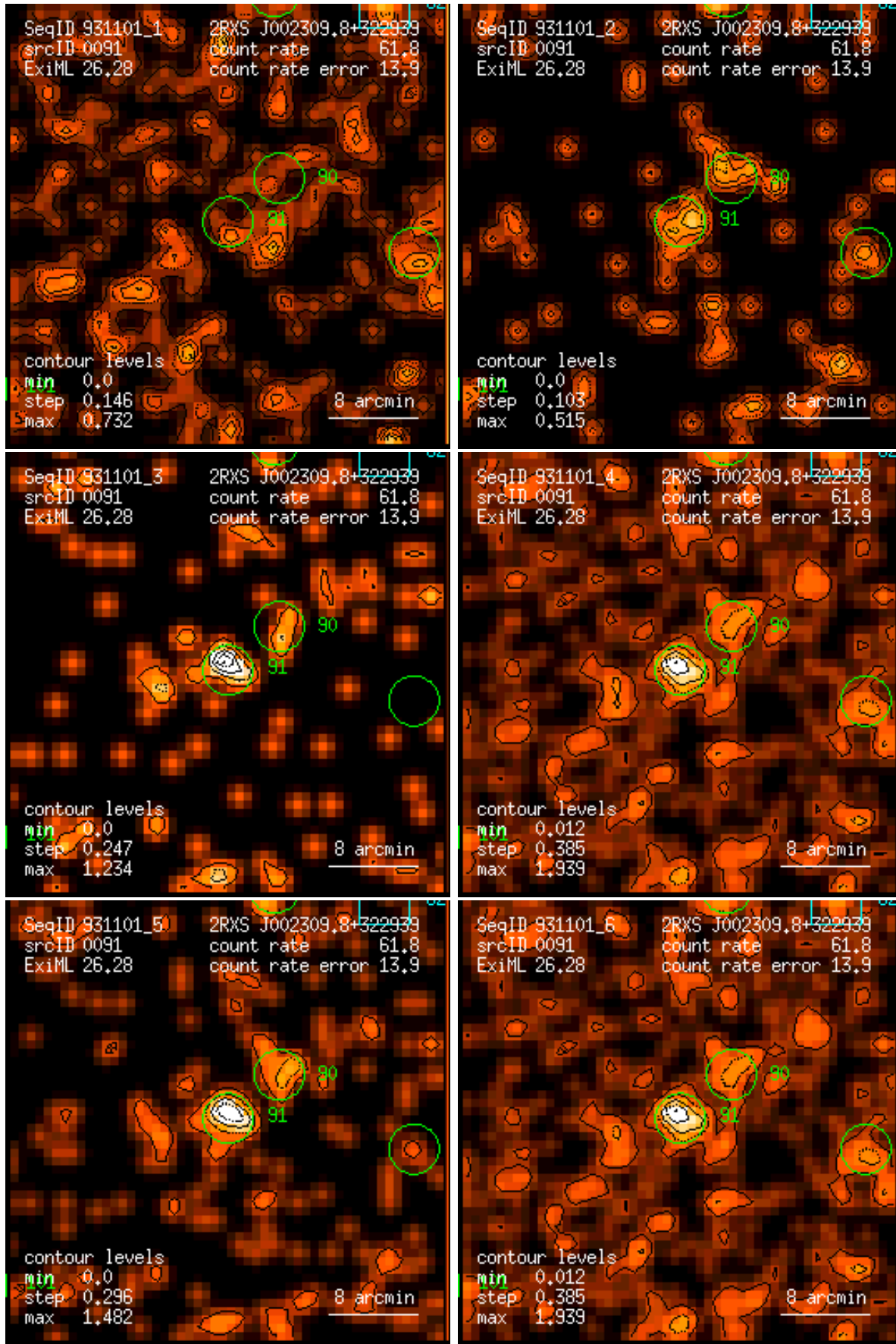
Figure 91: RASS 931101: detection 0091: band rate images, Gaussian filter: (1) PSPC channels 11 – 41, (2) 52 – 90, (3) 91 – 201, (4) 11 – 235, (5) 52 – 201, (6) 11 – 201. Broad band rates in counts/ks. Band rate contour levels in counts/ks/arcmin 2 .
