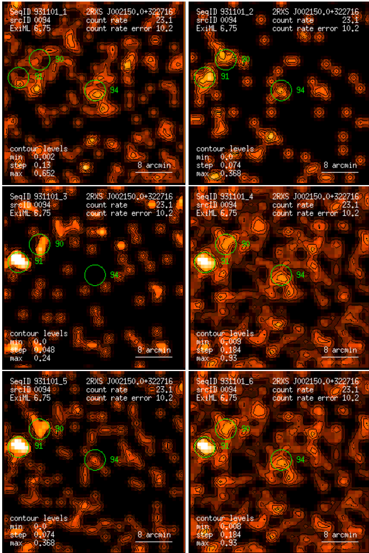
Figure 94: RASS 931101: detection 0094: band rate images, Gaussian filter: (1) PSPC channels 11 – 41, (2) 52 – 90, (3) 91 – 201, (4) 11 – 235, (5) 52 – 201, (6) 11 – 201. Broad band rates in counts/ks. Band rate contour levels in counts/ks/arcmin 2 .
