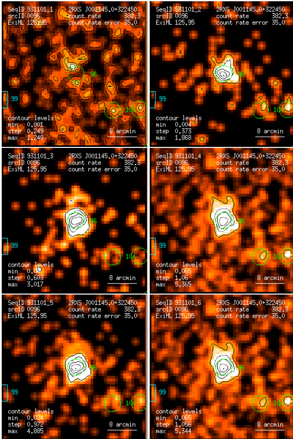
Figure 96: RASS 931101: detection 0096: band rate images, Gaussian filter: (1) PSPC channels 11 – 41, (2) 52 – 90, (3) 91 – 201, (4) 11 – 235, (5) 52 – 201, (6) 11 – 201. Broad band rates in counts/ks. Band rate contour levels in counts/ks/arcmin 2 .
