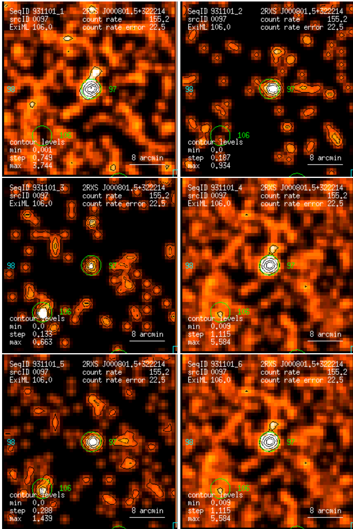
Figure 97: RASS 931101: detection 0097: band rate images, Gaussian filter: (1) PSPC channels 11 – 41, (2) 52 – 90, (3) 91 – 201, (4) 11 – 235, (5) 52 – 201, (6) 11 – 201. Broad band rates in counts/ks. Band rate contour levels in counts/ks/arcmin 2 .
