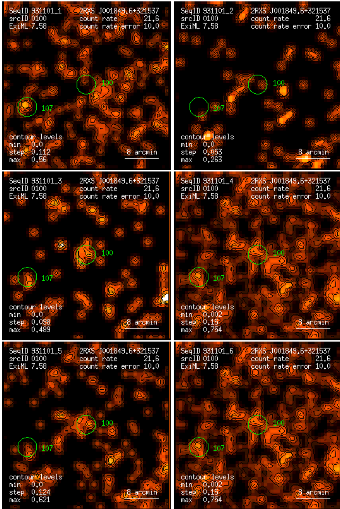
Figure 100: RASS 931101: detection 0100: band rate images, Gaussian filter: (1) PSPC channels 11 – 41, (2) 52 – 90, (3) 91 – 201, (4) 11 – 235, (5) 52 – 201, (6) 11 – 201. Broad band rates in counts/ks. Band rate contour levels in counts/ks/arcmin 2 .
